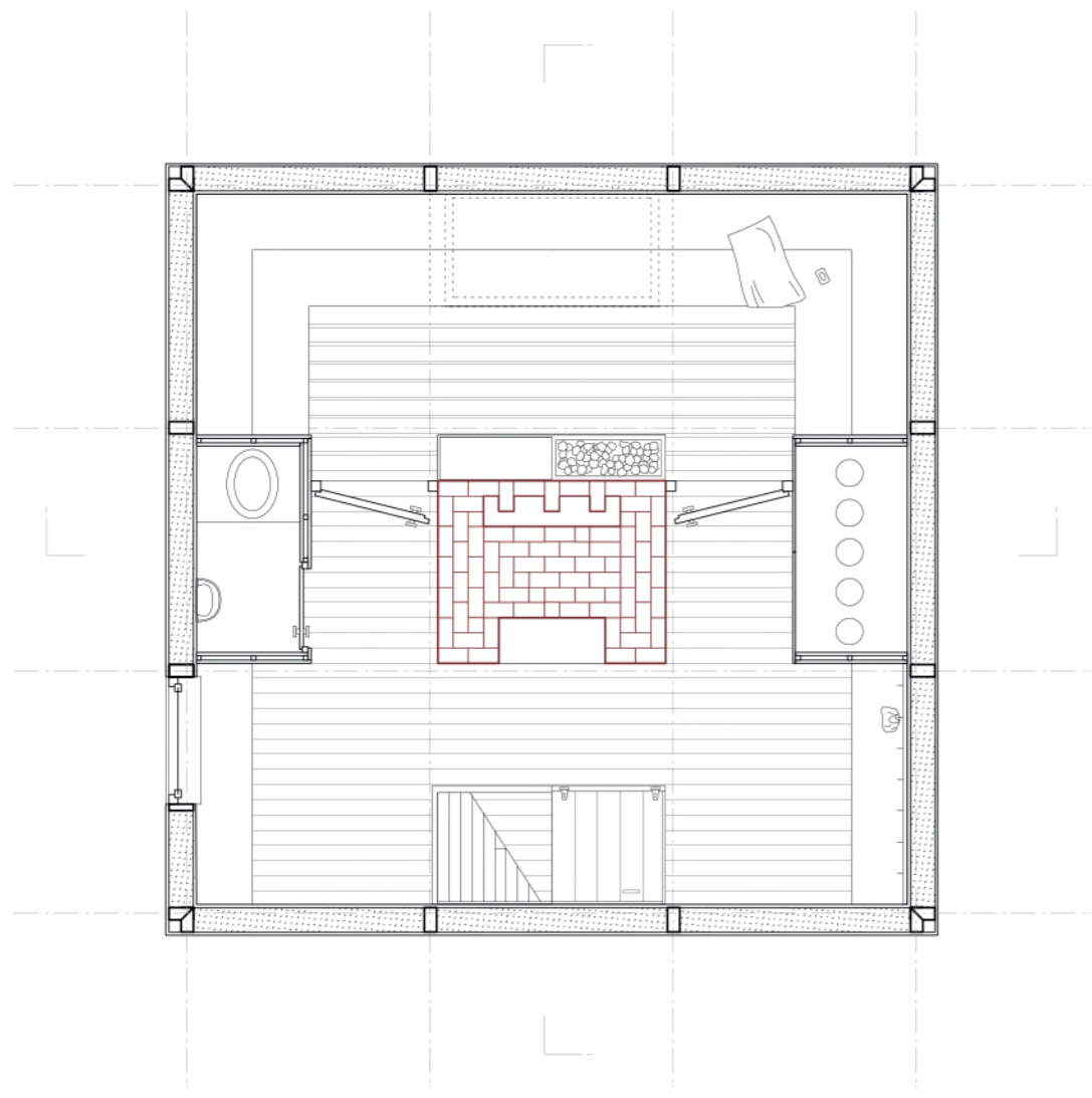
Plans 1/50
