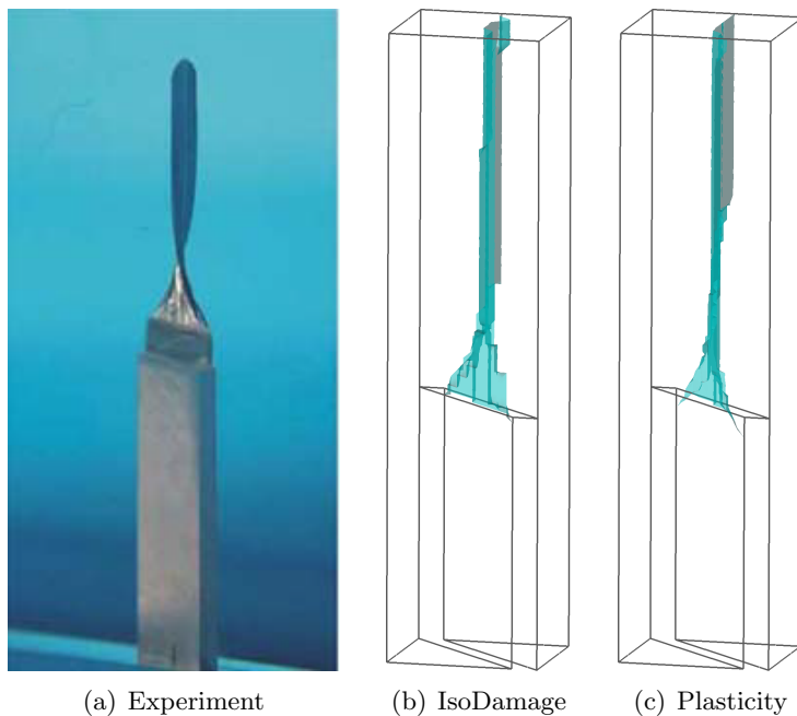
Figure 6: Experimental [10] and numerical ( \epsilon - u formulation) crack surface of the three point bending test on PMMA.
