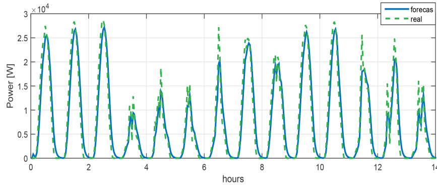
Figure 35.4: Solar power profile, forecasted vs. real.
