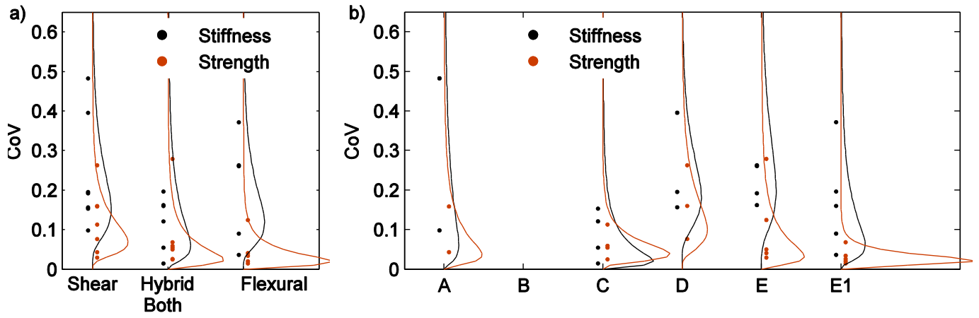
Fig. 7 Coefficients of variation of replicate tests for effective stiffness K_{eff} ultimate strength V_u as a function of the failure mode (a) and the masonry typology (b).
