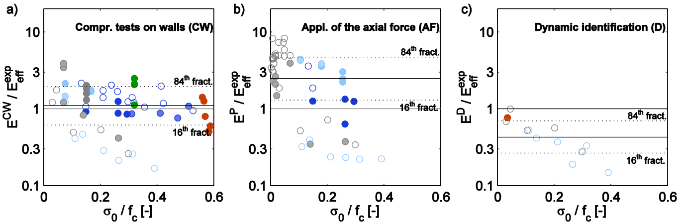
13 Fig. 11 Estimate of the effective stiffness for different experimental test: compression test on walls (a), stiffness measured 14 during the application of the axial force before the shear-compression test (b), and dynamic identification tests (c).
