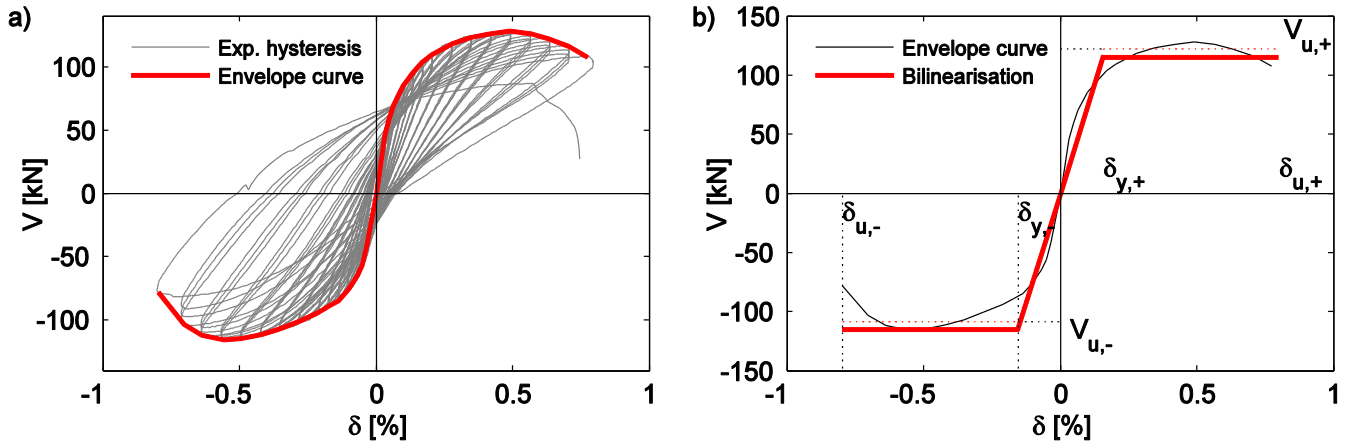
19 20 Fig. 3 Example of a force-displacement response curve (a) and definition of effective stiffness, strength and drift capacity 21 based on the envelope of the response (b).
