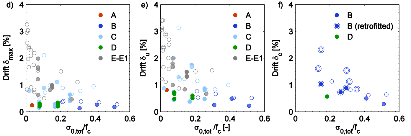
Fig. 16 Influence of the axial load ratio on the drift capacity at different limit states: a) Drift at the onset of cracking \delta_{cr} ; b) Drift at yield \delta_y ; c) Drift at maximum force \delta_{max} ; d) Drift limit “Significant damage” \delta_{SD}=\min(3\delta_{cr}, \delta_{max}) ; e) Drift at ultimate LS \delta_u ; f) Drift at collapse \delta_c . Solid markers represent walls failing in shear or a hybrid mode; empty markers walls failing in flexure. Note: The scale of the y-axis of plot a and b is different from those in plots c-f.
