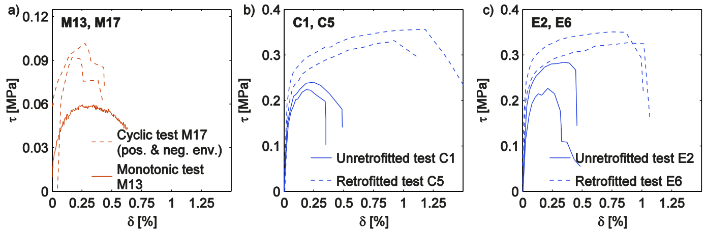
13 14 Fig. 9 Comparison of force-displacement relationship of monotonic and cyclic tests (a) and strengthened and 15 unstrengthened test units (b, c).
