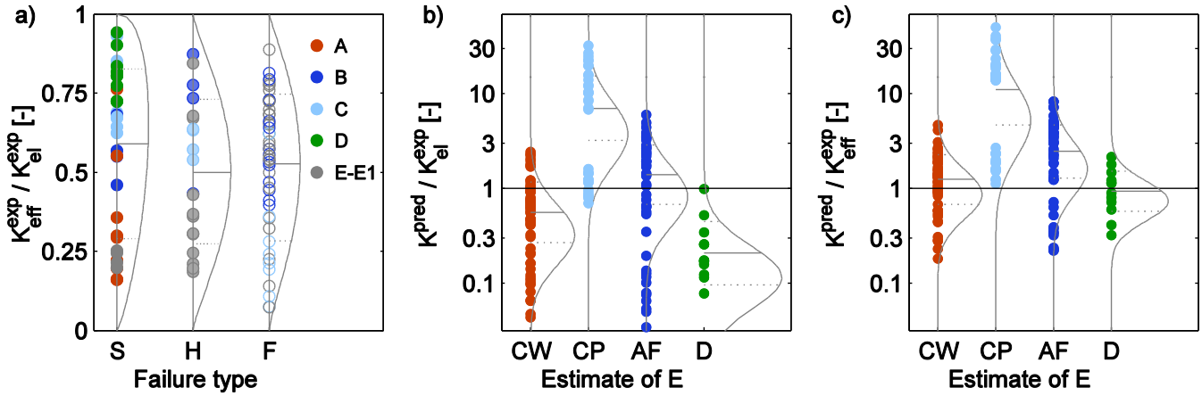
8 Fig. 10 Stiffness of walls subjected to horizontal loads: Effective to elastic wall stiffness ratios for different failure types and 9 masonry typologies (a); estimate of the experimental elastic wall stiffness (b) and effective wall stiffness (c) from different 10 types of tests (CW- compression tests on walls; CP – compression tests on prisms; AF – stiffness measured when applying 11 the axial force at the beginning of the shear-compression test; D – dynamic identification tests).
