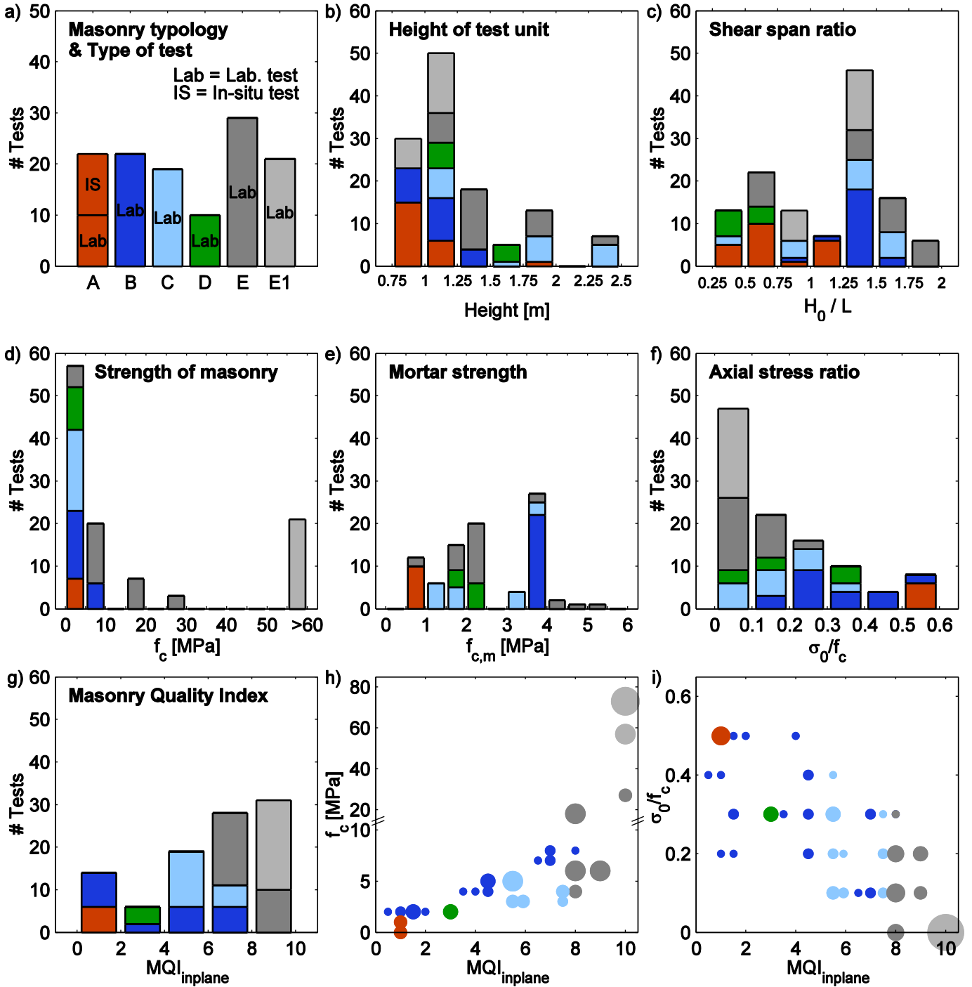
Fig. 4 Database of shear-compression tests on stone masonry walls: Distribution with regard to various parameters. The colours refer to the masonry typology (see plot a). For plots h) and i), the size of the marker relates to the number of test units with the corresponding parameter combination.
