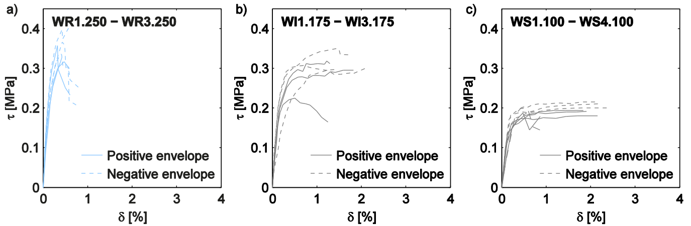
Fig. 6 Force-displacement envelopes of repeated tests by Vasconcelos and Lourenço (2009): Walls of masonry typology C (a), E (b) and E1 (c).
