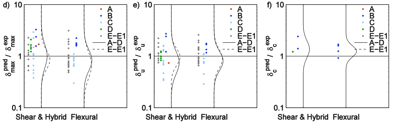
Fig. 19 Drift capacity model 1: Ratios of predicted to experimental drift capacities for the six different limit states.
