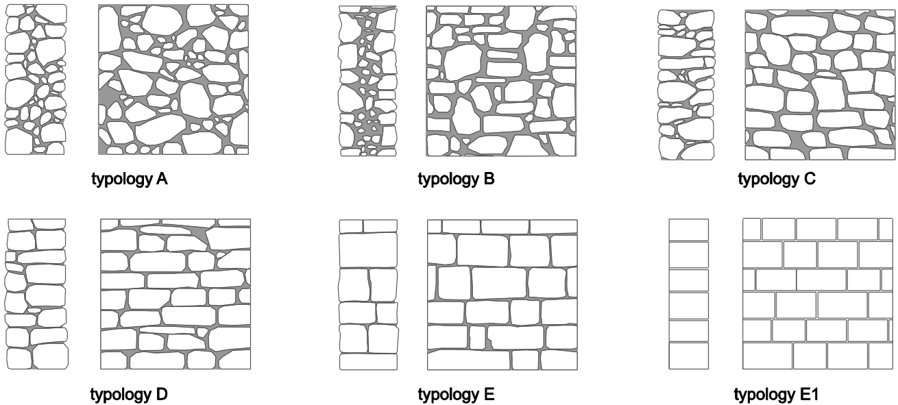
10 Fig. 2 Stone masonry typologies: sketches of typical textures and cross sections
