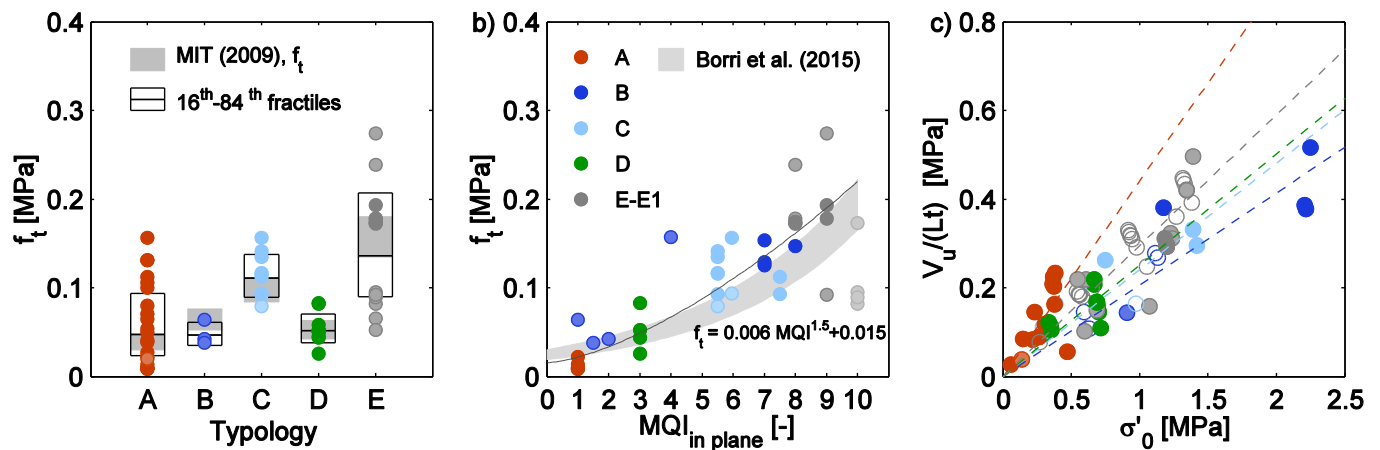
Fig. 14 a) Masonry tensile strength according to Turnšek-Čačovič criterion: comparison with ranges suggested in the Italian code (MIT 2009); b) Estimate of the experimental tensile strength from the Masonry Quality Index; c) Regression analysis for the estimation of the friction coefficient; the cohesive contribution is subtracted, assuming c = 2\mu f_t . The x-axis is derived from Eq. (8): \sigma'_0 = \sigma_0 + 3f_t - 6 \frac{VH_0 f_t}{\sigma_0 L^2 t} where V_u = \mu \cdot \sigma'_0 \cdot Lt .
