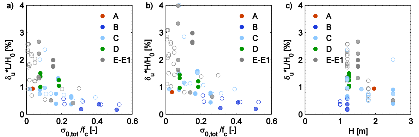
Fig. 17 Ultimate drift capacity \delta_u : Normalising the drift capacity by L/H_0 (a) and H/H_0 (b). Influence of the wall size on the drift capacity (c).
