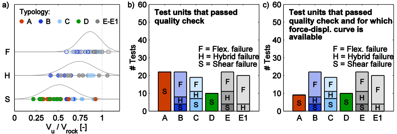
12 Fig. 5 Quality check of shear-compression tests on stone masonry walls: Ratio of maximum shear strength to rocking 13 strength (a), distribution of all tests that passed the quality check (b), distribution of all tests that passed the quality check 14 and for which the force-displacement curve is available. 15
