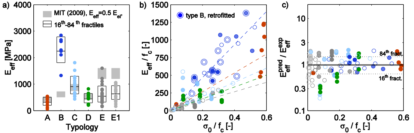
6 7 Fig. 12 Comparison between the experimental effective stiffness and the ranges proposed in the Italian code; b) relation 8 between effective stiffness and axial load, normalized to the compressive strength f_c ; c) prediction of the effective stiffness 9 through Eq. (6).
