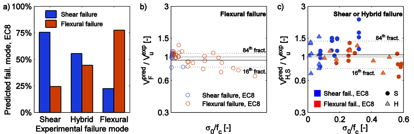
30 31 Fig. 13 a) Failure mode predicted by Eurocode 8 part 3; b) Estimate of the flexural capacity; c) Estimate of the shear 32 capacity according to EC8-3 (Mohr-Coulomb criterion on the uncracked length of the section).
