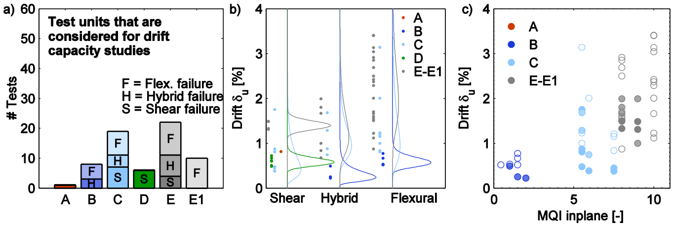
16 17 Fig. 15 Distribution of test units considered for drift capacity studies (a). Ultimate drift capacity \delta_u as a function of the 18 failure mode (b), and the Masonry Quality Index for in-plane loading (c). Solid markers represent walls failing in shear or 19 a hybrid mode; empty markers walls failing in flexure.
