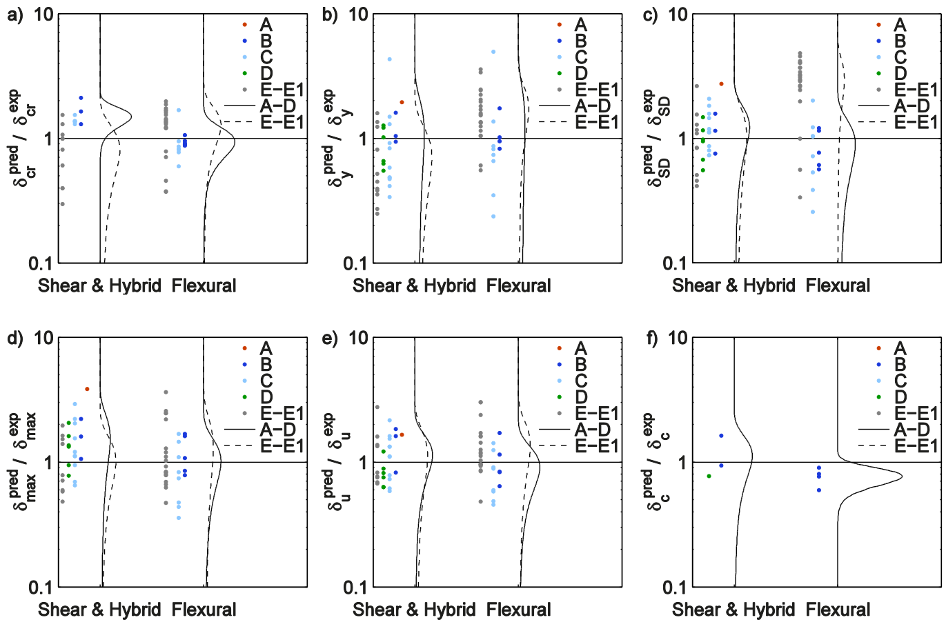
Fig. 21 Drift capacity model 2: Ratios of predicted to experimental drift capacities for the six different limit states.
