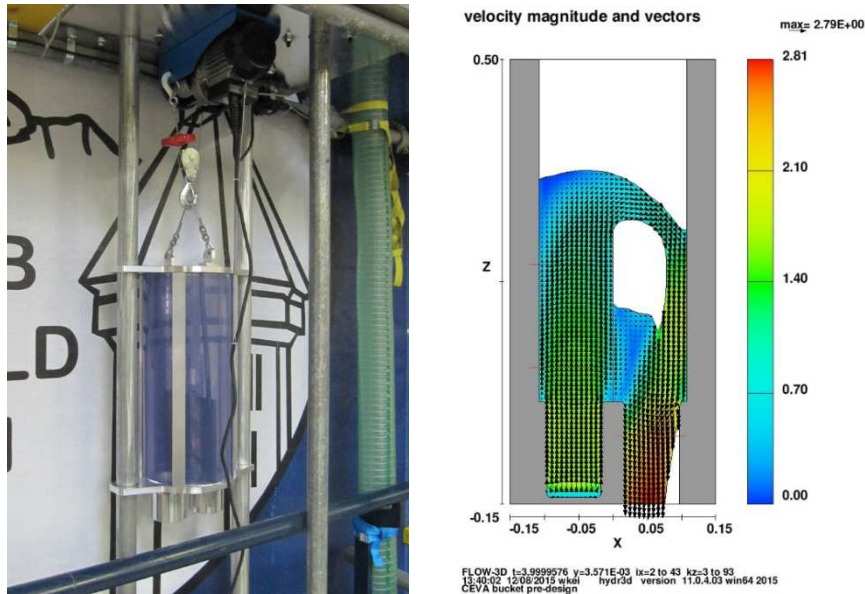
Figure 3: Image of the mobile bucket and the motor (left). Image of the numerical simulation done with Flow 3D (right).
