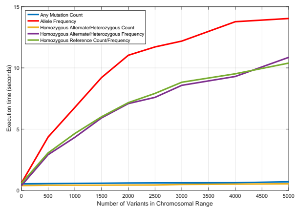
Fig. 6: Total execution time at i2b2 server per number of consecutive genetic variants.
