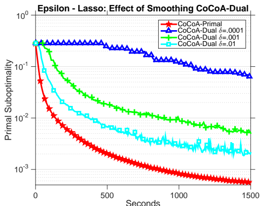
Figure 3 & Table 6: For pure L_1 regularization, Nesterov smoothing is not an effective option for CoCoA in the dual. It either modifies the solution (Figure 3) or slows convergence (Table 6). This motivates running CoCoA instead on the primal for these problems.
