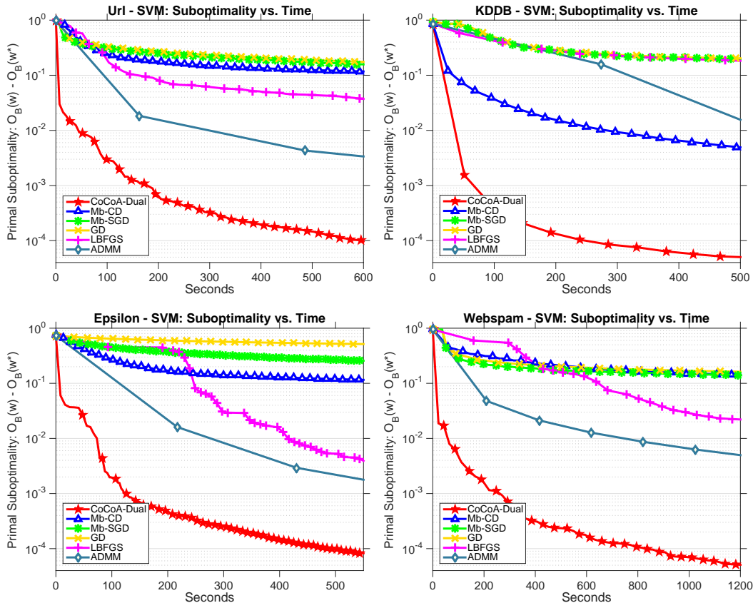
Figure 3: Suboptimality in terms of \mathcal{O}_B(\mathbf{w}) for solving a hinge-loss support vector machine model: url ( K=4 , \lambda=1E-4 ), kddb ( K=4 , \lambda=1E-6 ), epsilon ( K=8 , \lambda=1E-5 ), and webspam ( K=16 , \lambda=1E-5 ) datasets. CoCoA applied to the dual formulation converges more quickly than all other compared methods in terms of the time in seconds.
