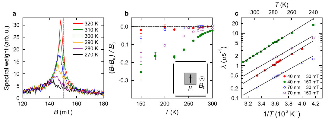
Figure 4. Transverse muon-spin rotation data. (a) Fourier spectra measured in an applied field of B_0 = 150 mT for a 40-nm-thick film of FeGe L . Evolution with temperature of (b) the diamagnetic shift and (c) the relaxation rate \lambda for the two FeGe films at two values of the applied field B_0 . Temperature-activated behaviour is evident above T = 260 K, as described in the text.
