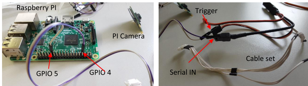
Fig. 4. Connection between FLIR Tau 2 camera and the Raspberry Pi computer.
