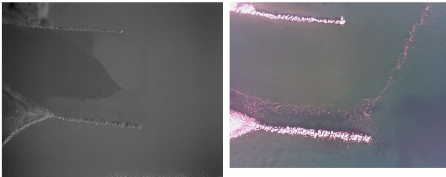
Fig. 13. Discharge of the Venoge River into Lake Geneva. The left image shows the disappearance of the river discharge due to negative buoyancy in the inflow. The right image shows the accompanying RGB camera picture (with NIR filter removed).
