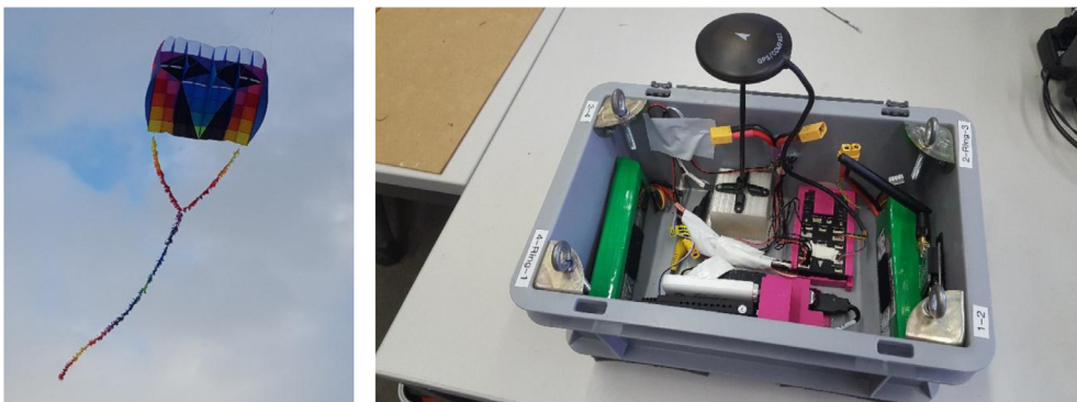
Fig. 10. Kite (left) and the ImPROV imagery package (right) used with it.
