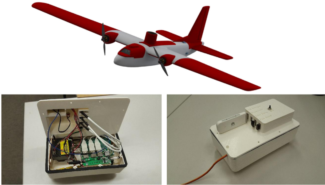
Fig. 12. Long range UAV (top) with adapted ImPROV package (bottom, assembled with 3D-printed pieces). The ImPROV package is installed in the fuselage with cameras pointing vertically downwards.
