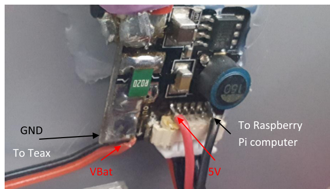
Fig. 9. Modified battery monitor.
