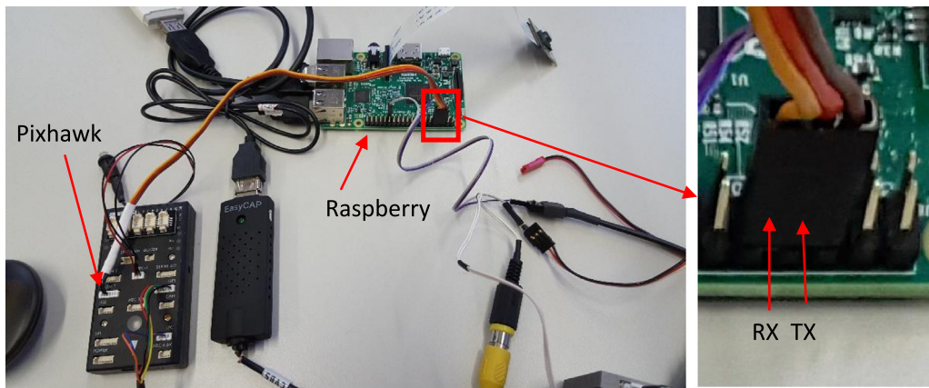
Fig. 8. Autopilot connected to the Raspberry Pi computer.
