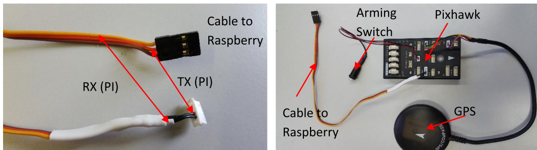
Fig. 7. Essential components connected to the Pixhawk autopilot: GPS, serial to the Raspberry Pi computer, arming switch.
