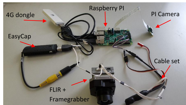
Fig. 6. Overall setup showing connections between the FLIR and Raspberry Pi cameras, and the LTE communication dongle, to the Raspberry Pi computer.
