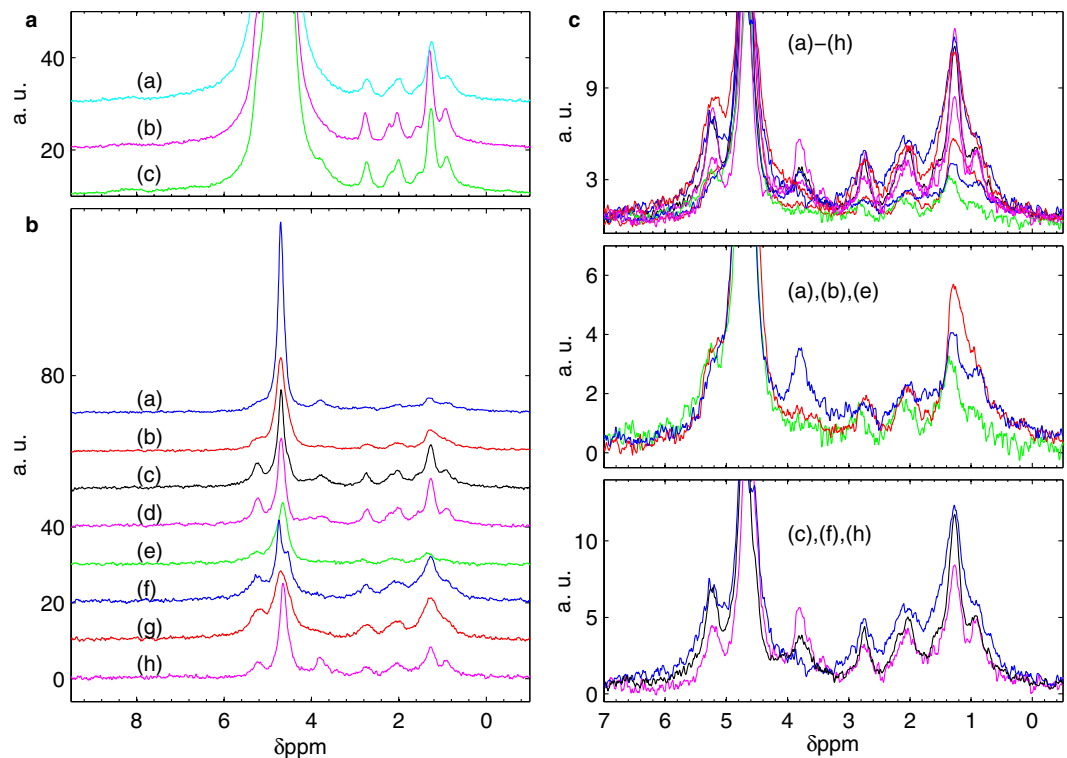
Figure 2. NMR spectroscopy of single Richtersius coronifer ( Rc ) ova. (a) Three Rc single ovum experiments in H 2 O-based gels realized by dispersing 1.5% agarose in either M9 buffer (a) or pure H 2 O (b–c). (b) Eight Rc single ovum experiments in D 2 O-based gels realized by dispersing 1.5% agarose in pure D 2 O. (c) Detailed comparison of Rc ova in D 2 O-based gels. Colors refer to the same spectra as in (b).
