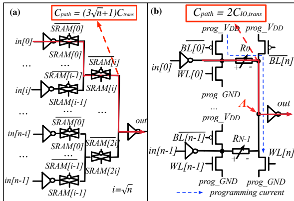
Fig. 1. Schematics and path capacitances of (a) SRAM-based and (b) RRAM-based multiplexers.
