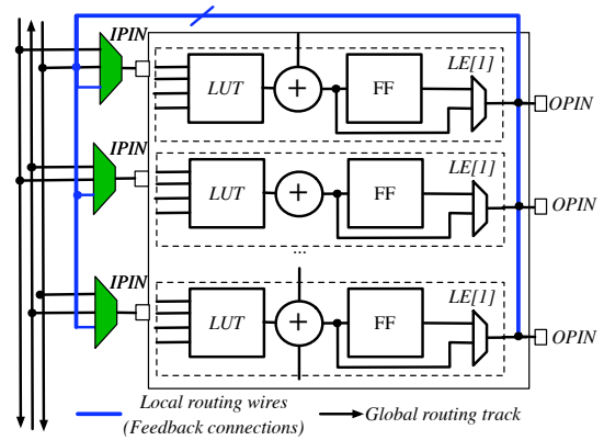
Fig. 2. Proposed CB and CLB architectures.
