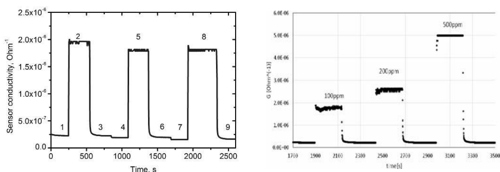
Fig. 4. (Left) Sensor response to 100 ppm of hydrogen at different values of relative humidity (RH): 1 – air @ 80%; 2 – 100 ppm H 2 @ 80%; 3 – air @ 80%; 4 – air @ 60%; 5 – 100 ppm H 2 @ 60%; 6 – air @ 60%; 7 – air @ 40%; 8 – 100 ppm H 2 @ 40%; 9 – air @ 40%. (Right) Sensor response to different concentrations of hydrogen at RH = 60%.
