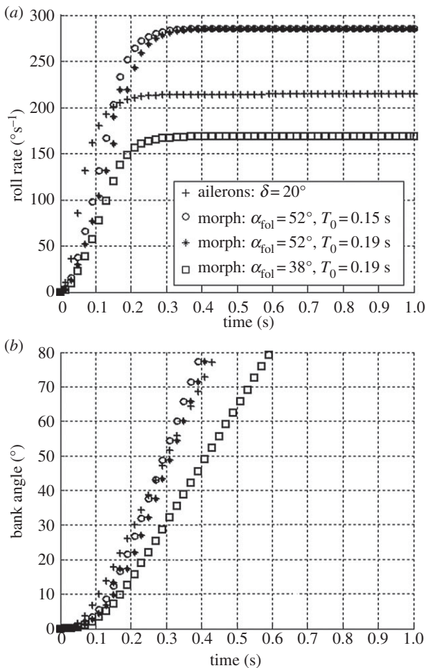
Figure 8. Maximum roll rate and bank angle comparison: ailerons ( \delta = 20^\circ ) and asymmetric morphing ( \alpha_{\text{fol}} = 52^\circ ) for T_o corresponding to a load factor of 0 and 4. The value I_{xx} = 0.010 \text{ kg m}^{-2} is used in the simulations which corresponds to the inertia of the morphing prototype with fully open wing.
