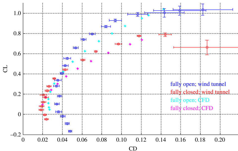
Figure 6. Polar curves for the morphing wing in the fully open and fully folded configurations ( Re 70 000). The computational curves (cyan and magenta) has been obtained combining the lift distribution obtained in AVL simulations with the polar curves for the two-dimensional aerofoils computed with XFOIL (the morphing wing fully open is used as reference surface). Polar curves of the morphing wing at Re 70 000 obtained through wind tunnel measurements (blue and red).
