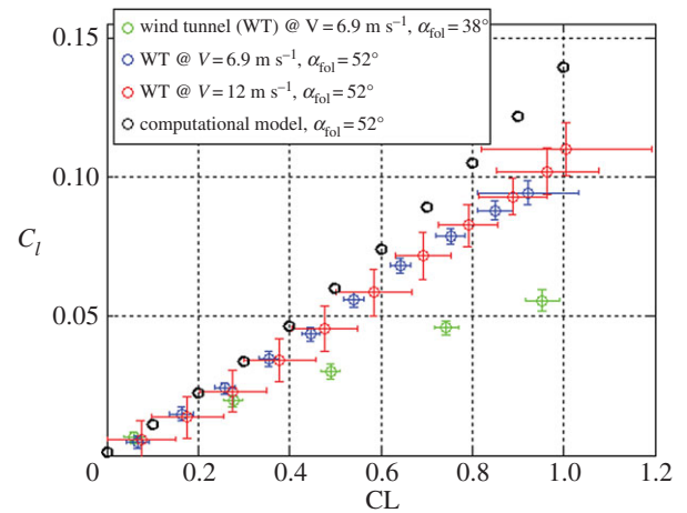
Figure 9. Roll torque coefficient as a function of CL: one semi-wing fully open while the other is folded at an angle \alpha_{\text{fol}} = 52^\circ for two different speeds (blue, red) and 38^\circ (green). The results of the computational model for \alpha_{\text{fol}} = 52^\circ are in black.
