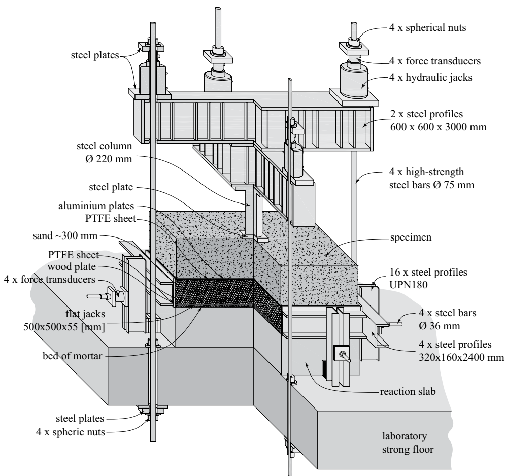
Fig. 4. Schematic representation of test setup
