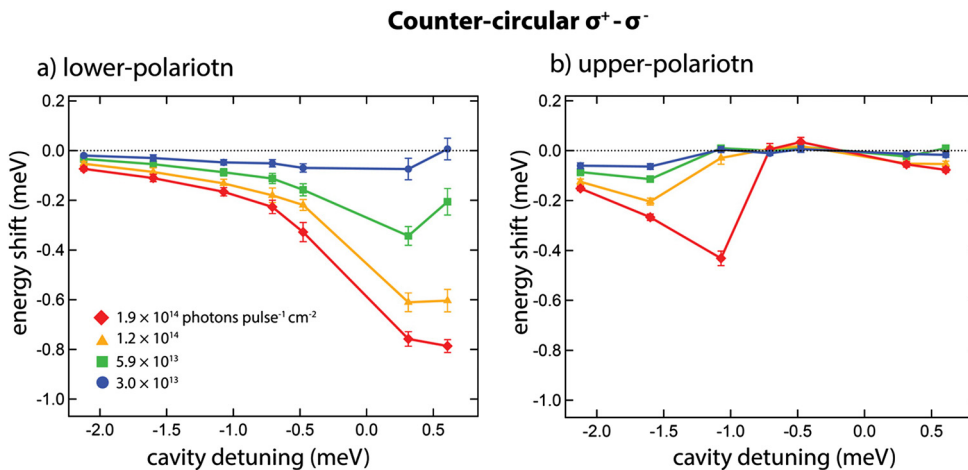
Fig. 11. Energy shifts of (a) lower and (b) upper polaritons in counter-circular excitation, as a function of cavity detuning. Four different symbols represent the different pump intensities. From the PhD thesis of Naotomo Takemura [49].
