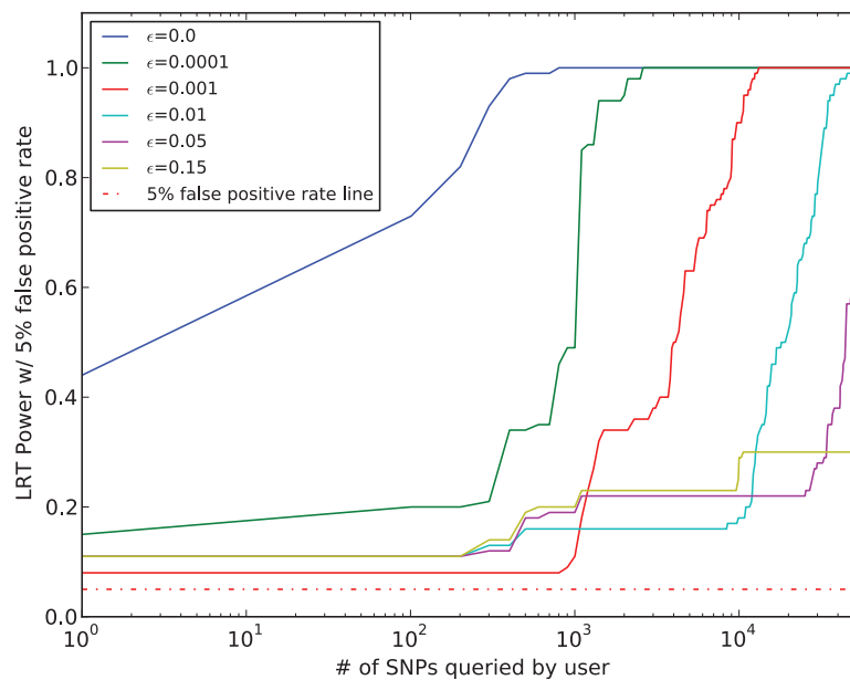
Figure 4. “Optimal” re-identification attack in beacon with S2 . Different power rates per number of SNPs queried (with rare-first logic) from a beacon with mitigation S2 by an adversary with knowledge on \epsilon and on AFs from the 1000 Genomes project. Different colors for different values of \epsilon .
