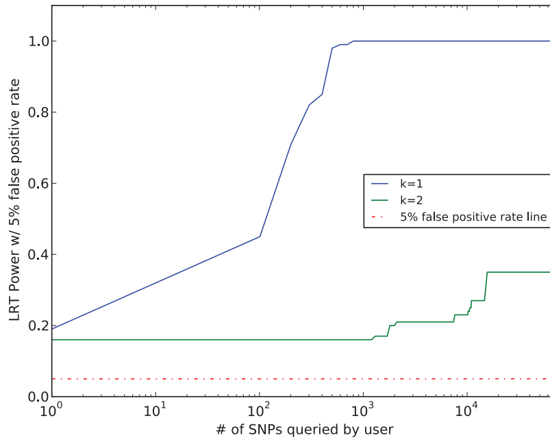
Figure 3. “Optimal” re-identification attack in beacon with S1 . Different power rates per number of SNPs randomly queried from a beacon with mitigation S1 by an adversary with knowledge on k and on AFs from the 1000 Genomes project: (blue) k = 1 ; (green) k = 2 .
