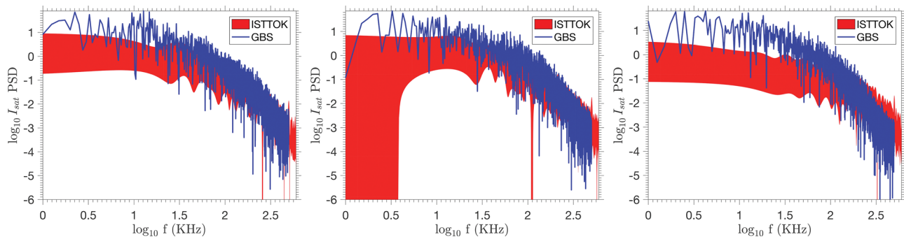
FIG. 12. I_{sat} power spectra from the experiment (red) and simulations (blue), at r - a = 0 mm (left), r - a = 5 mm (center), and r - a = 10 mm (right).
