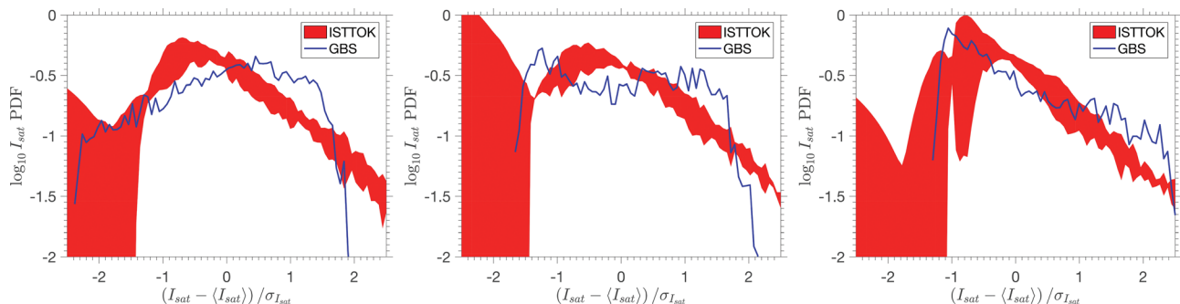
FIG. 10. I_{sat} PDF from the experiment (red) and simulation (blue), at r - a = 0 mm (left), r - a = 5 mm (center), and r - a = 10 mm (right).
