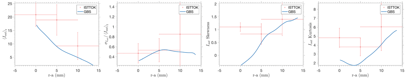
FIG. 9. Statistical moments of I_{sat} from the experiment (red) and simulation (blue). From left to right: mean, standard deviation, skewness, and kurtosis.
