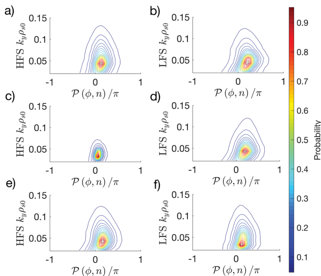
FIG. 6. Phase-shift probability between density and electric potential fluctuations, resulting from GBS simulations with standard ISTTOK parameters (top), and when DW (middle) or BM (bottom) are removed from the system. The HFS (left) and LFS (right) are shown.
