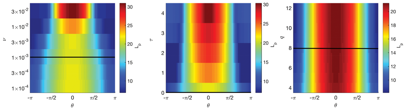
FIG. 7. Equilibrium pressure scale-length, L_p , as a function of the poloidal angle \theta and normalised resistivity, \nu (left panel), ion to electron temperature ratio, \tau (middle panel), and safety factor, q (right panel). The black lines represent the standard ISTTOK case.
