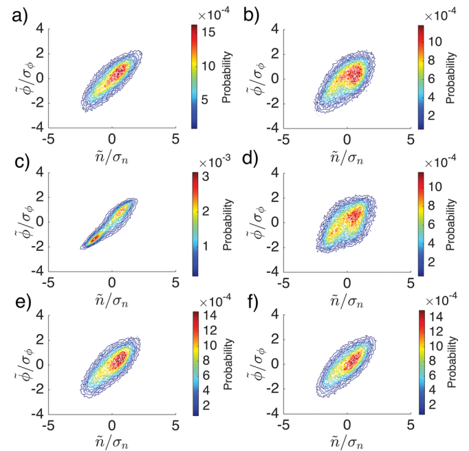
FIG. 5. Probability of correlation between density and electric potential fluctuations normalized to their respective standard deviation, resulting from GBS simulations with standard ISTTOK parameters (top), and when DW (middle) or BM (bottom) are removed from the system. The HFS (left) and LFS (right) are shown.
