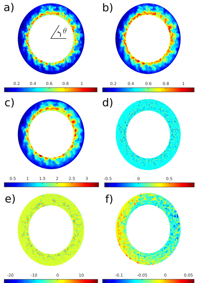
FIG. 1. Snapshots of plasma turbulence in the standard ISTTOK simulation on a poloidal cross section halfway between the limiter plate ( \varphi = \pi ). We show: (a) plasma density n/n_0 , (b) electron temperature T_e/T_{e0} , (c) electrostatic potential \phi/eT_{e0} , (d) vorticity \omega = \rho_{s0}^2 \nabla_{\perp}^2 \phi/eT_{e0} , (e) electron V_{\parallel e}/c_{s0} , and (f) ion V_{\parallel i}/c_{s0} parallel velocities.
