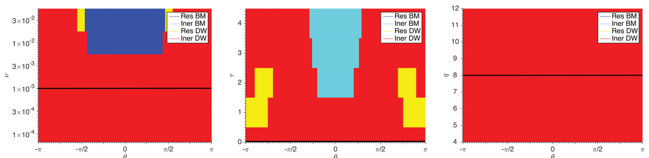
FIG. 8. Turbulent regimes as a function of the poloidal angle \theta and normalised resistivity, \nu (left panel), ion to electron temperature ratio \tau (middle panel), and safety factor q (right panel). The Resistive BM driven turbulence is in dark blue, Inertial BM in light blue, Resistive DW in yellow, and Inertial DW in red. The black lines represent the standard ISTTOK case.
