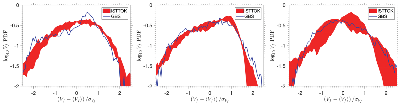
FIG. 11. V_f PDF from the experiment (red) and simulation (blue), at r - a = 0 mm (left), r - a = 5 mm (center), and r - a = 10 mm (right).
