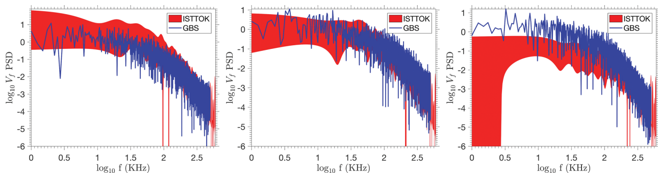
FIG. 13. V_f power spectra from the experiment (red) and simulations (blue), at r - a = 0 mm (left), r - a = 5 mm (center), and r - a = 10 mm (right).
