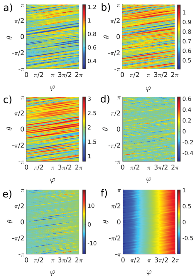
FIG. 2. Snapshots of plasma turbulence for the standard ISTTOK simulation on a toroidal cross section at x = x_s + 5 \rho_{s0} . We show: (a) plasma density n/n_0 , (b) electron temperature T_e/T_{e0} , (c) electrostatic potential \phi/eT_{e0} , (d) vorticity \omega = \rho_{s0}^2 \nabla_{\perp}^2 \phi/eT_{e0} , (e) electron V_{||e}/c_{s0} , and (f) ion V_{||i}/c_{s0} parallel velocities.
