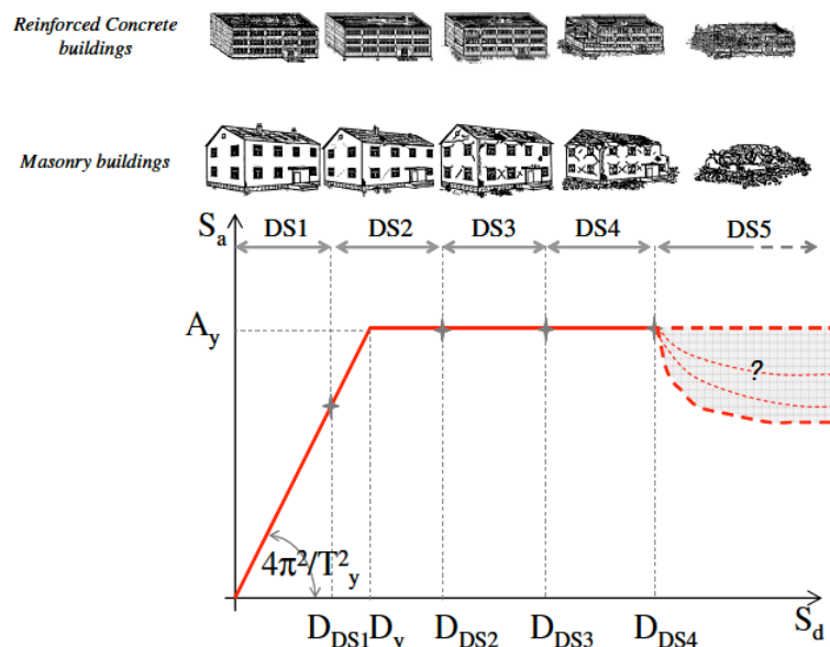
Figure 11 : Capacity curve according to Displacement Based Vulnerability method and definition of damage limit state. [28]
