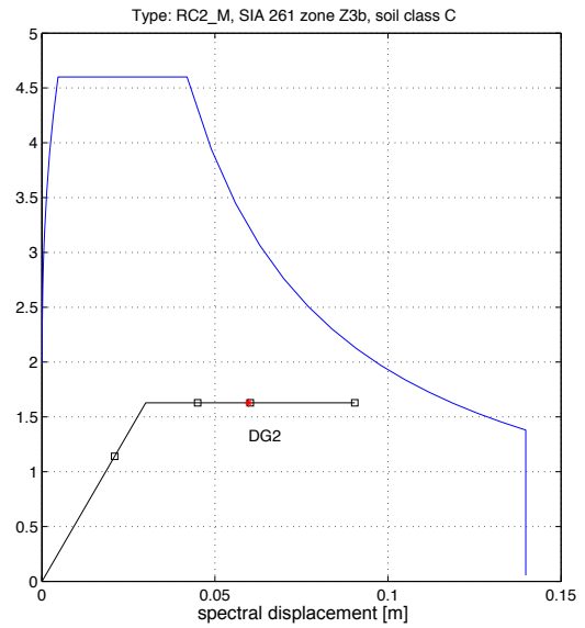
Figure 22 : Comparison: results for 5-storey building of typology C and RC2_M.
