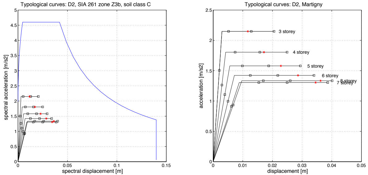
Figure 19 : Typical curves for the specific typology D2 and the performance point related to response spectrum of soil class C and seismic zone Z3b [25].
