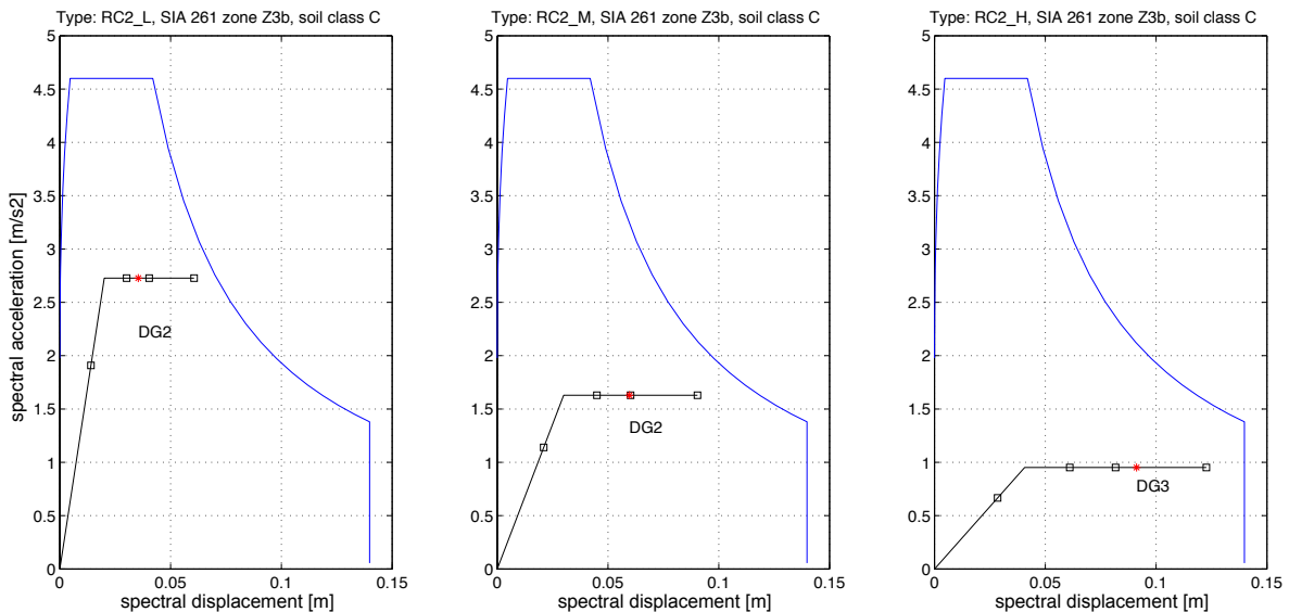
Figure 20 : Method LM2: damage grade of RC2 typology for soil class C and seismic zone Z3b.
