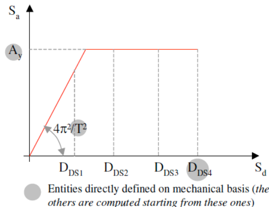
Figure 12 : Capacity curve definition for unreinforced masonry buildings. [28]
