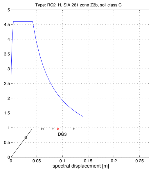
Figure 23 : Comparison: results for 8-storey building of typology C and RC2_H.
