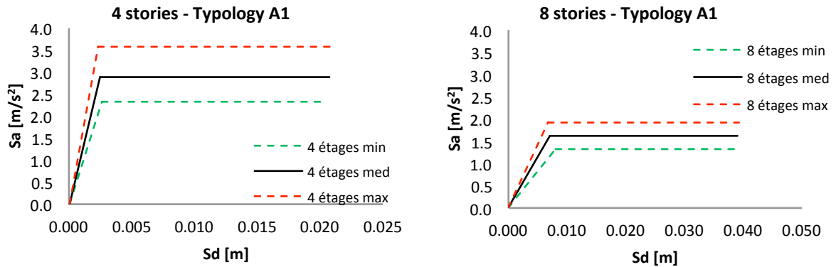
Figure 15 : Typology A1, minimal, mean and maximal typological curves for buildings of 4 and 8 stories. [27]
