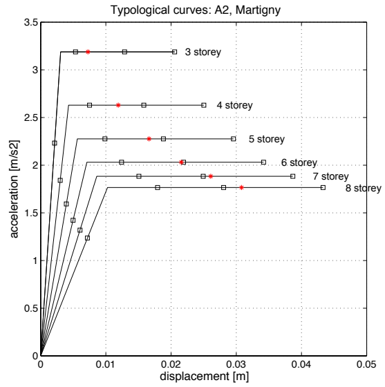
Figure 17 : Typological curves for the specific typology A2 and the performance point related to response spectrum of soil class C and seismic zone Z3b [25].
