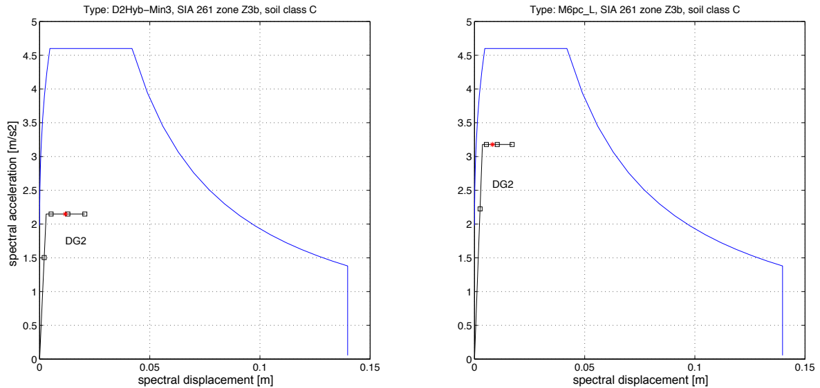
Figure 24 : Comparison: results for 3-storey building of typology D2 and M6-PC_L.
