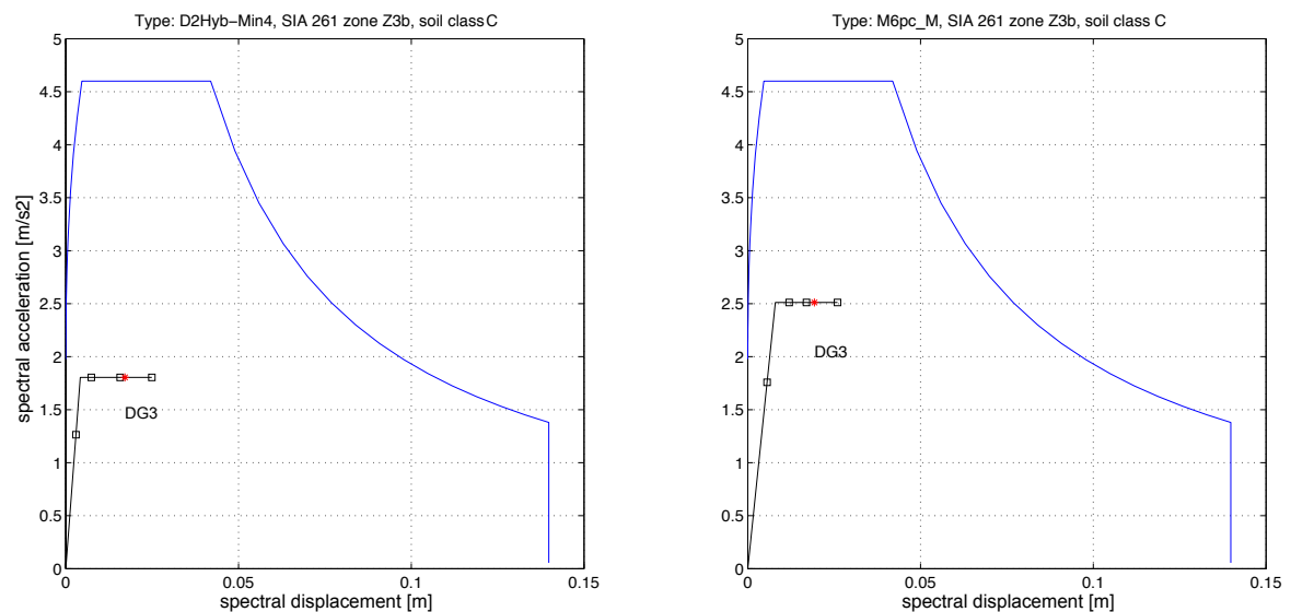
Figure 25 : Comparison: results for 4-storey building of typology D2 and M6-PC_M.
