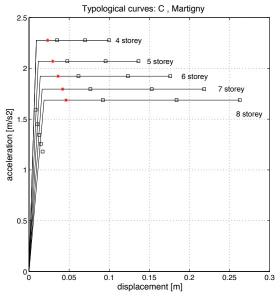
Figure 18 : Typological curves for the specific typology C and the performance point related to response spectrum of soil class C and seismic zone Z3b [25].
