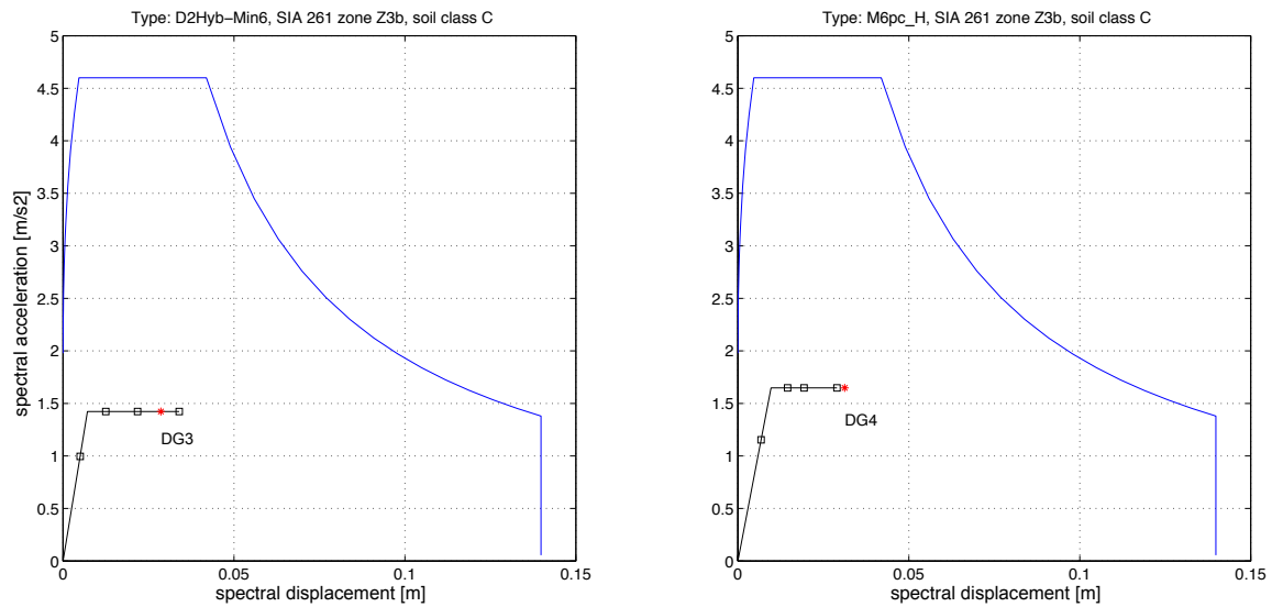
Figure 26 : Comparison: results for 6-storey building of typology D2 and M6-PC_H.
