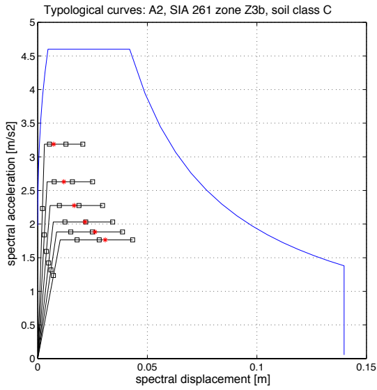
Figure 17 : Typological curves for the specific typology A2 and the performance point related to response spectrum of soil class C and seismic zone Z3b [25].
