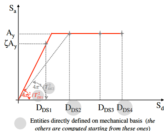
Figure 13 : Capacity curve definition for reinforced concrete buildings. [28]
