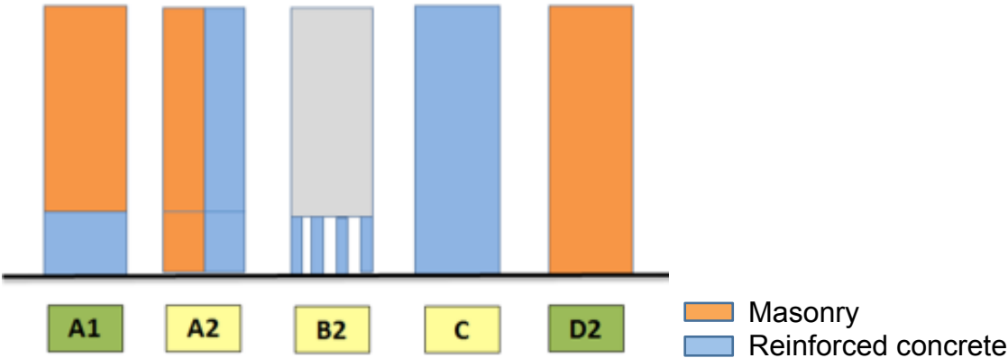
Figure 8 : Specific typology for typical Swiss buildings [27].
