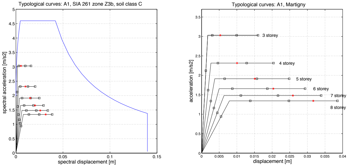
Figure 16 : Typological curves for the specific typology A1 and the performance point related to response spectrum of soil class C and seismic zone Z3b [25].
