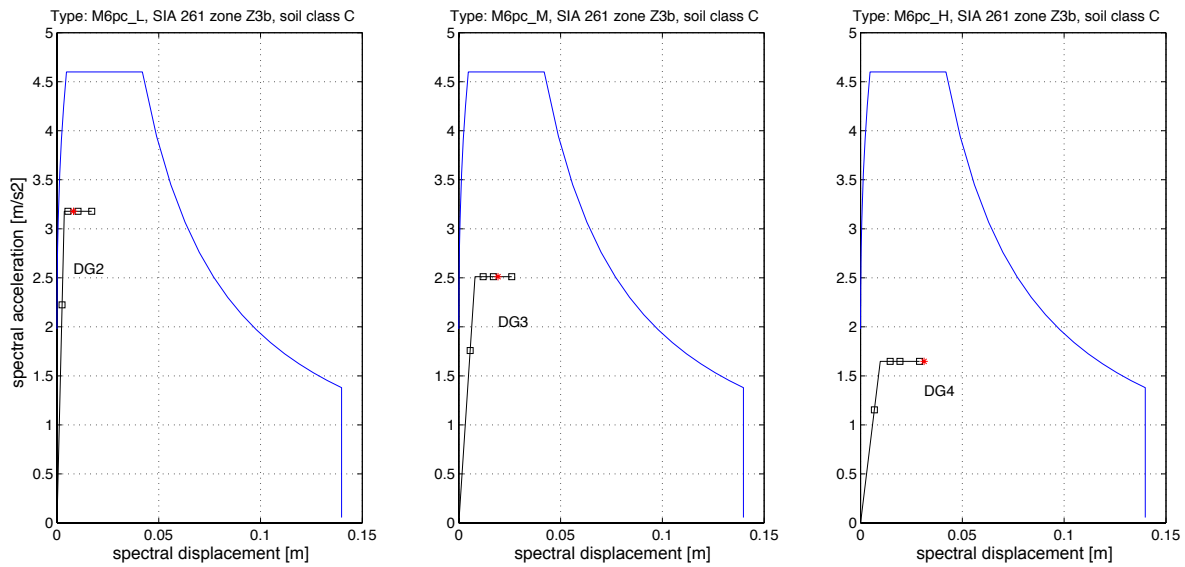
Figure 21 : Method LM2: damage grade of M6-PC typology for soil class C and seismic zone Z3b.
