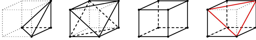
Fig. 1: The first three polytopes (the simplex, the cross-polytope and the cube) are clearly 2-level. The fourth one is not 2-level, due to the highlighted facet.
