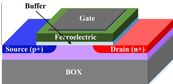
Fig. 1. The device schematic of an SOI Fe-TFET where the gate stack of a conventional single gate TFET is replaced with a series combinations of a ferroelectric and a linear dielectric.
