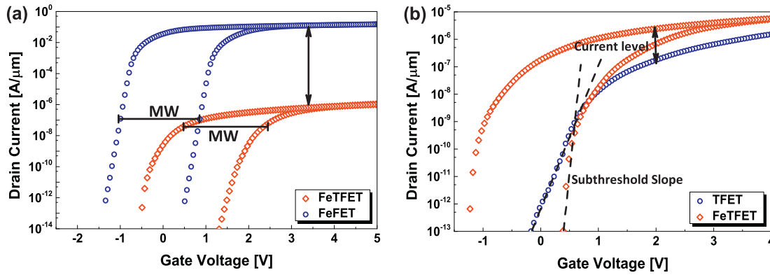
Fig. 8. (a) The transfer characteristic of a 28 nm gate length FeFET vs. Fe-TFET using 10 nm of Si:HfO 2 as the ferroelectric. The drain voltage is considered 1 V for all simulations which is the supply voltage of the 28 nm ITRS node. Results confirm that the Fe-TFET provides the same memory window as the FeFET with lower power consumption. (b) The negative capacitance effect enhances the output current level and subthreshold slope of the Fe-TFET comparing the conventional TFET. Results are obtained using Sentaurus TCAD commercial simulator.
