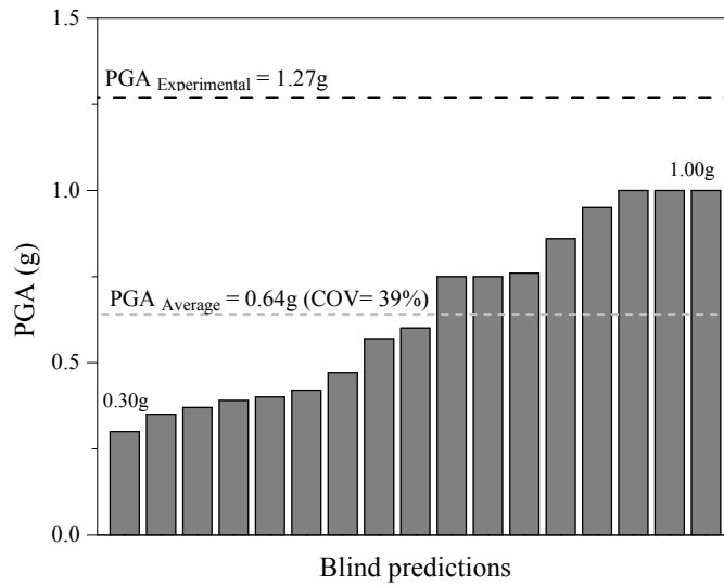
Figure 11 – PGA for all blind predictions of the brick structure.
