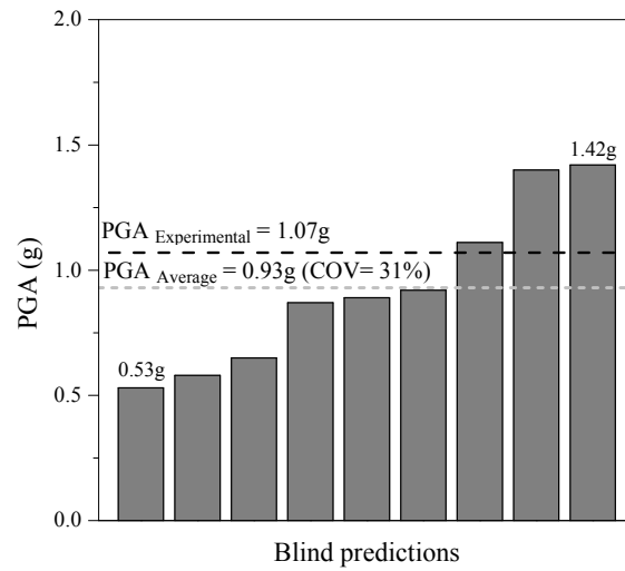
Figure 9 – PGA for the good blind predictions of the stone structure.
