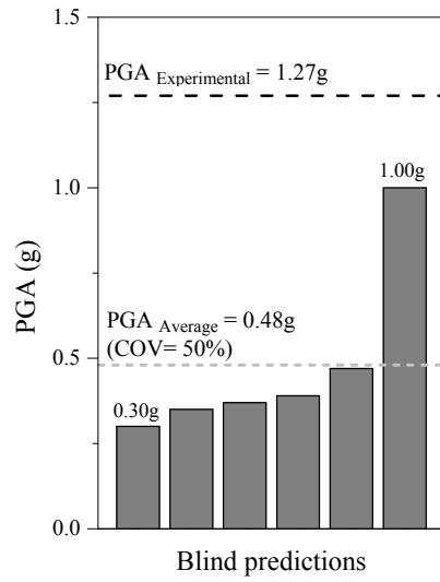
Figure 12 – PGA for the fair blind predictions of the brick structure.
