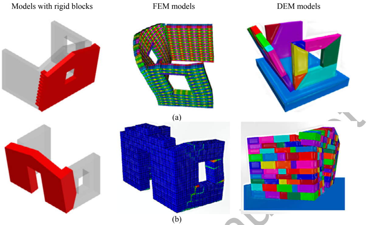
Figure 6 – Examples of models developed by the experts: (a) brick structure; (b) stone structure.
