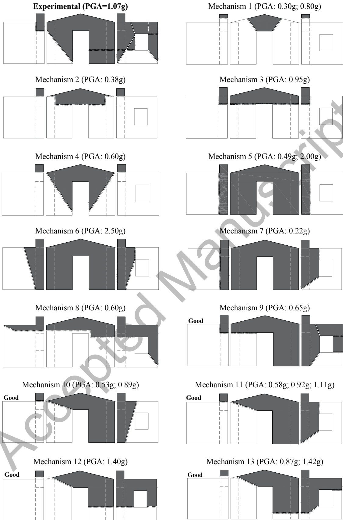
Figure 7 – Idealized collapse mechanisms for the stone structure.
