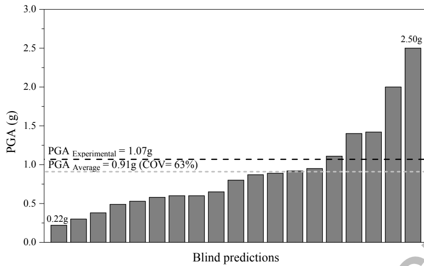
Figure 8 – PGA for all blind predictions of the stone structure.
