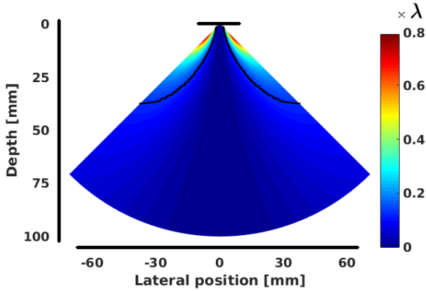
Fig. 2. Error map derived from the travel time equivalence between a sectorial acquisition using DW and the equivalent PW imaging after the application of the proposed spatial transformation. The computed error is expressed relatively to the wavelength used in the experiments. The black line on the top of the figure models the transducer location while the axis origin is located at the center of the probe. The two black curves drawn inside the error map represent the boundary of the region at the edge of the image where the maximum error is higher than \lambda/8 .
