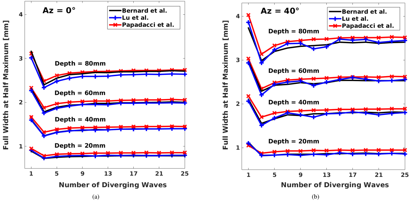
Fig. 5. Numerical phantom - lateral resolution measurements as a function of the number of DWs computed at 20-mm, 40-mm, 60-mm and 80-mm at (a) the middle of the image (azimuth angle of 0°) and (b) at the edge of the image (azimuth angle of 40°).
