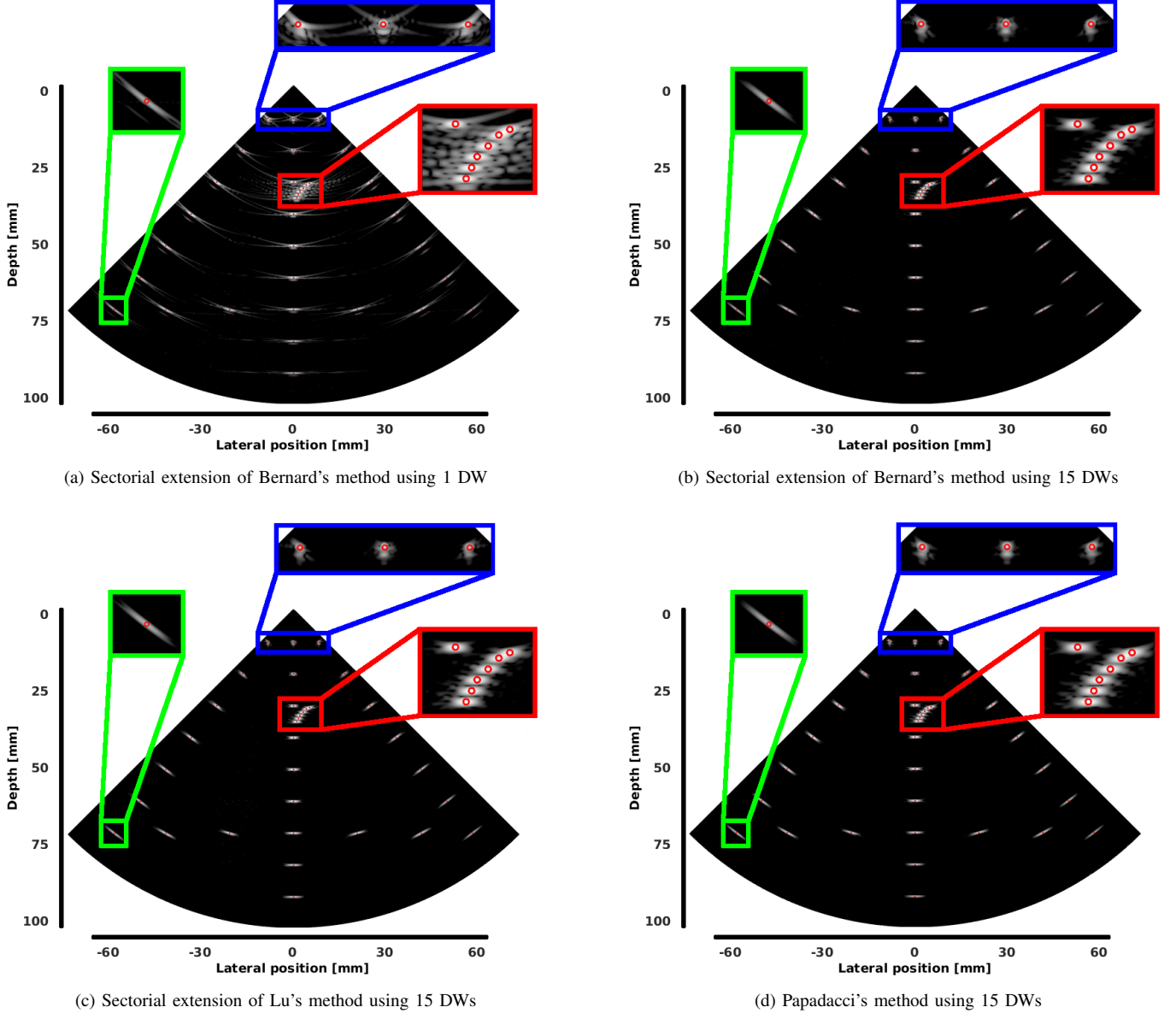
Fig. 4. Synthetic phantom reconstructed from the extension of the Fourier-based methods of Bernard et al. and Lu et al. as well as the method of Papadacci et al. The red points correspond to the real position of the scatterers involved in the simulation.
