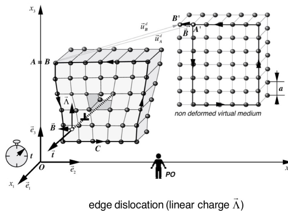
Figure 1 - screw and edge dislocations defined by their respective linear charge \Lambda and \vec{\Lambda}
