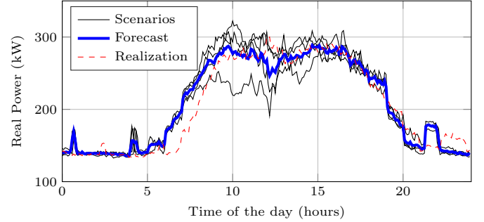
Fig. 5. Prosumption scenarios and forecast as computed by the forecasting tool compared with the realization.
