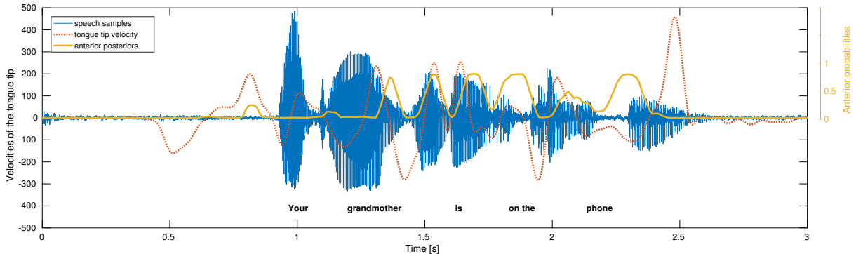
Figure 2: Anterior phonological posteriors vs. the electromagnetic articulography tongue tip measurement. Anterior posteriors were generated using analysis described in Section 4.1.2. The correlation between the articulatory gesture score and the trajectory of its corresponding phonological class posterior probability is evident.
