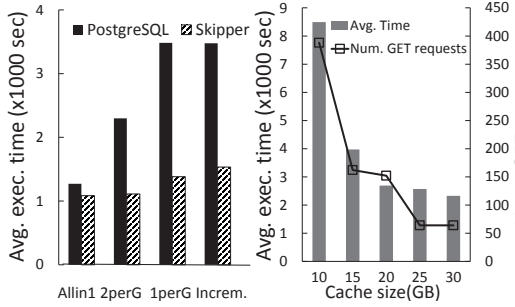
Figure 11: MJoin sensitivity to: a) layout b) cache size c) data set size
