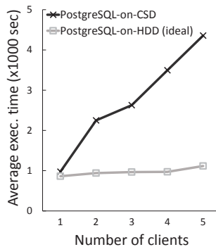
Figure 4: PostgreSQL over CSD vs HDD
