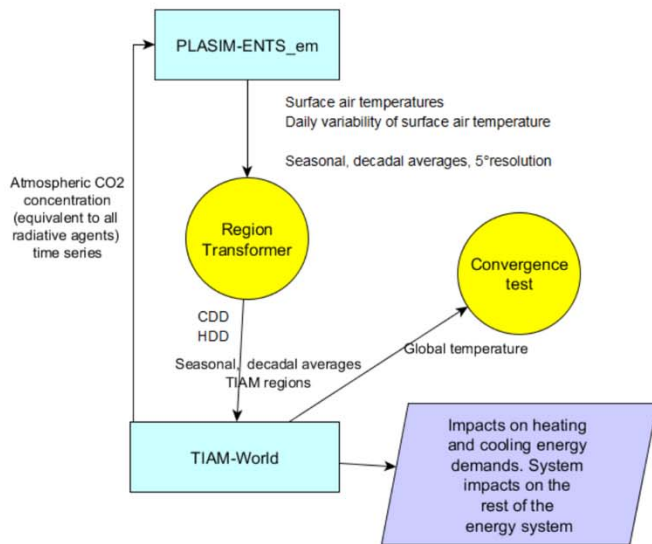
Fig. 5. The exchange of variables between models in the bespoke framework generator (BFG2) for the PLASIM-ENTSem_TIAM-WORLD coupling. This diagram is generated automatically from the BFG2. The circles denote transformers, the rectangles denote models and the parallelogram denotes outputs from the model. Arrows indicate the direction of data flow within the coupling.
