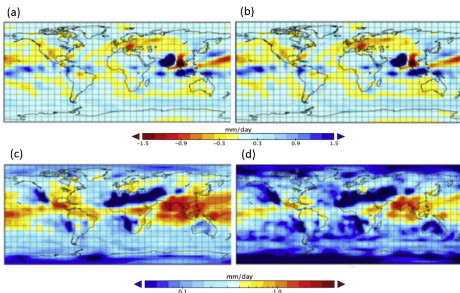
Fig. 2. The change in decadal-averaged June-July-August precipitation between 2000 and 2100 AD in response to RCP4.5 forcing: a) PLASIM-ENTS (simulated) ensemble mean, b) PLASIM-ENTS_em (emulated) ensemble mean, c) simulated ensemble standard deviation and d) emulated ensemble standard deviation. Note the logarithmic scale.
