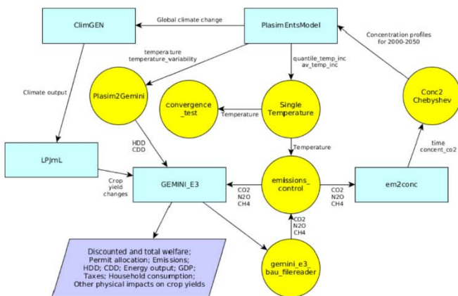
Fig. 3c. The exchange of variables between models in the bespoke framework generator (BFG2) for the PLASIM-ENTSem_ClimGEN_LPJmLem_GEMINI-E3 coupling. This diagram is generated automatically from the BFG2. The circles denote transformations, the rectangles denote models and the parallelogram denotes outputs from the model. Arrows indicate the direction of data flow within the coupling.
