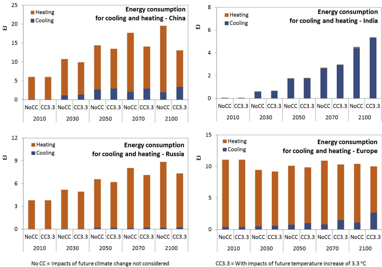
Fig. 9. Energy consumption for heating and cooling corresponding to a long-term global average temperature increase of 3.3 °C (Reference Case) - Focus on four countries.
