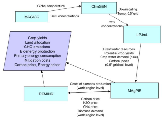
Fig. 4. The exchange of variables between models in the bespoke framework generator (BFG2) for the MAGICC_ClimGEN_LPJmL_MagPIE_REMIND coupling. This diagram is generated automatically from the BFG2. The rectangles denote models and the parallelogram denotes outputs from the model. Arrows indicate the direction of data flow within the coupling.
