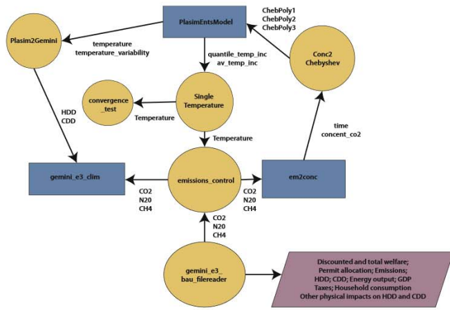
Fig. 3b. The exchange of variables between models in the bespoke framework generator (BFG2) for the PLASIM-ENTSem_GEMINI-E3 coupling. This diagram is generated automatically from the BFG2. The circles denote transformations, the rectangles denote models and the parallelogram denotes outputs from the model. Arrows indicate the direction of data flow within the coupling. Model names within these figures are slightly different from the text as they are program names for example: gemini_e3 is GEMINI-E3.
