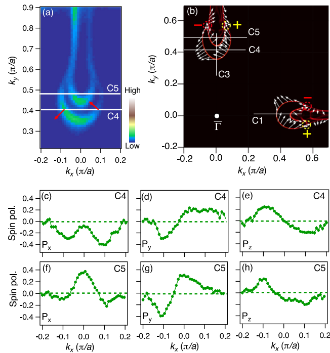
FIG. 3 (color online). (a) Spin-integrated FS map near \bar{\Gamma} - \bar{Y} recorded with the spin-resolved system at the COPHEE end station. The red arrows indicate the direction of measured in-plane spin polarizations of the Fermi arc b2 at C4 . (b) Corresponding theoretical spin texture of surface states, with white lines indicating the locations of the SARPES measurements, labeled as C1 , C3 , C4 , and C5 . Red and yellow dashed circles indicate the Weyl nodes W1 with negative and positive chirality, respectively. (c)–(e) Angle-resolved spin polarizations along C4 in the x , y , and z directions, respectively. (f)–(h) Same as (c)–(e), but along C5 . All the spectra in Fig. 3 were measured at h\nu = 36 eV with C -polarization and at a binding energy of 20 meV.
