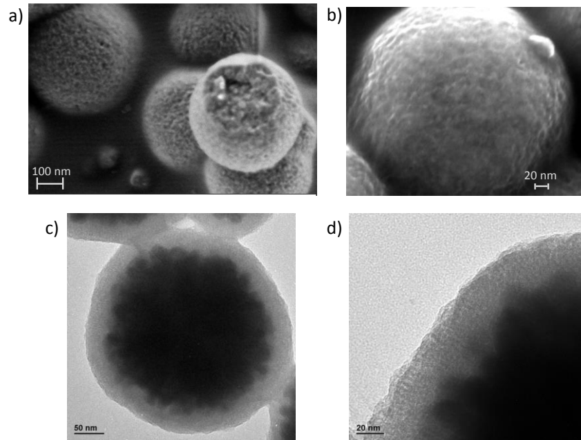
Figure SI-2. Images of the C_8-Fe_3O_4@mSiO_2 microspheres obtained by a) HR-SEM, 0.5 kV; b) HR-SEM, 5 kV; c) TEM at 120 kV; d) TEM at 120 kV, zoomed view.
