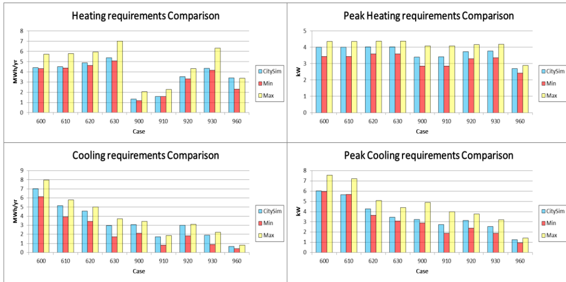
Fig. 5 - BESTEST results for the annual heating and cooling loads and the peak heating and cooling requirements
