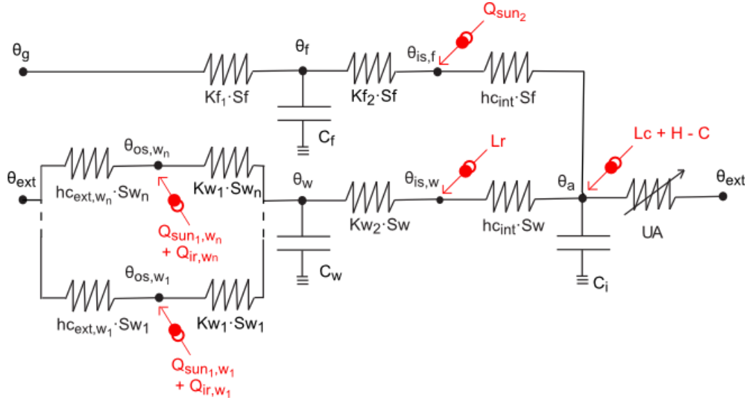
Fig. 1 - The four node thermal model as an equivalent electric circuit not showing the roof node for simplification (roof node similar to wall node)
