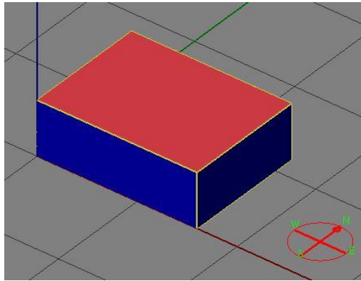
Fig. 2 - BESTEST base case geometry in CitySim Designer
