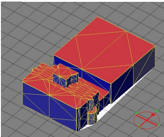
Fig. 3 – LE building in CitySim Designer
