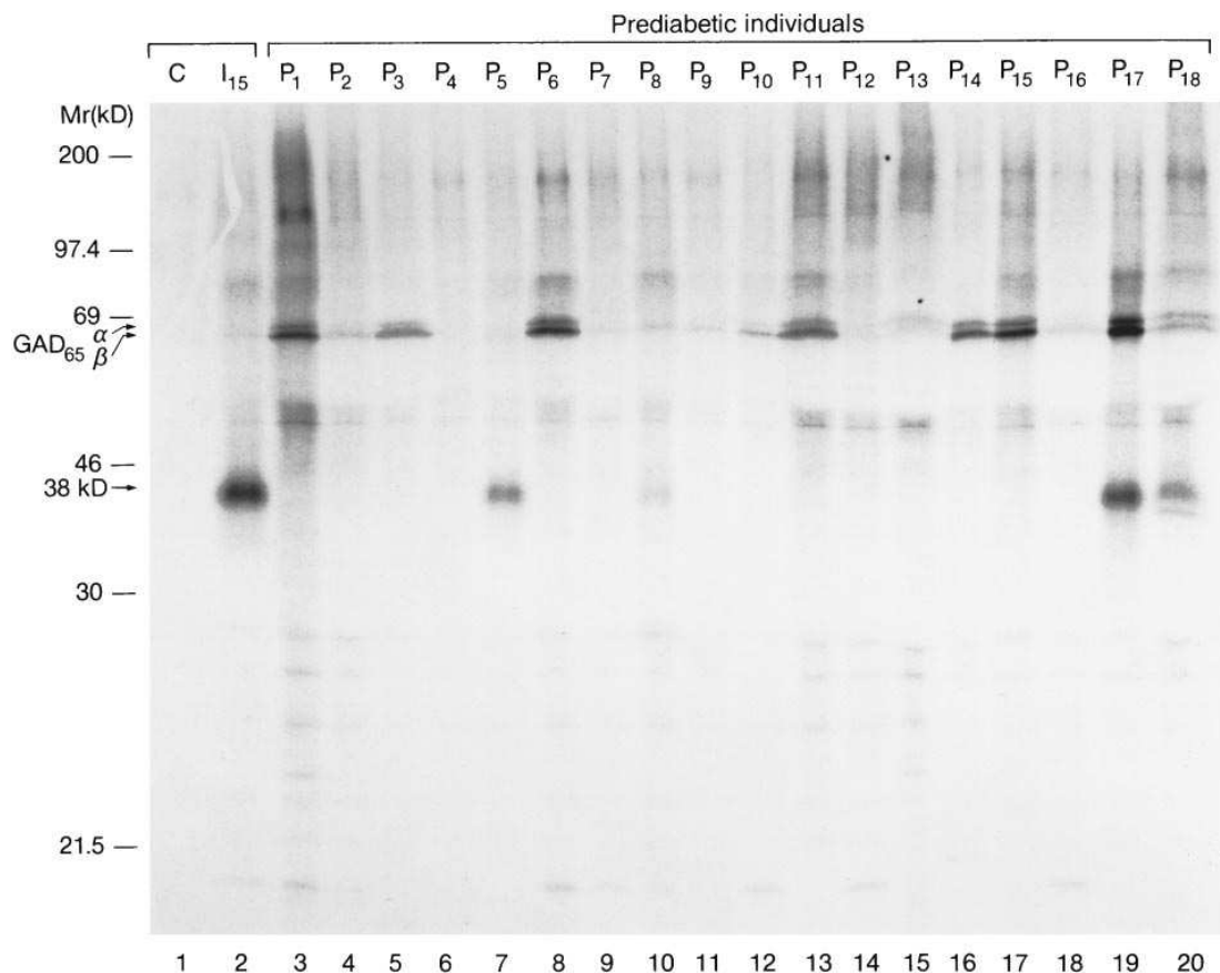
Figure 7. Analyses of 38-kD and GAD 65 autoantibodies in prediabetic individuals. Immunoprecipitation of membrane fractions of [ 35 S]methionine-labeled islet cell proteins with sera from prediabetic individuals P 1 –P 18 (lanes 3–21). The 38-kD protein is recognized by P 5 , P 8 , P 17 , and P 18 , 3, 33, 53, and 74 mo, respectively, before clinical onset of type 1 diabetes.
