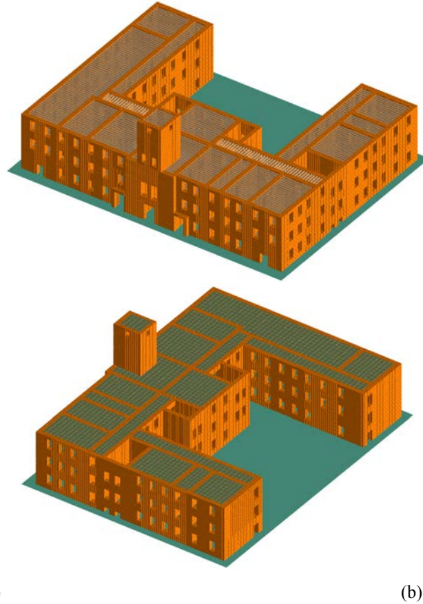
Figure 6: Three-dimensional numerical model of the building with view of timber beams and slab (Refined mesh).
