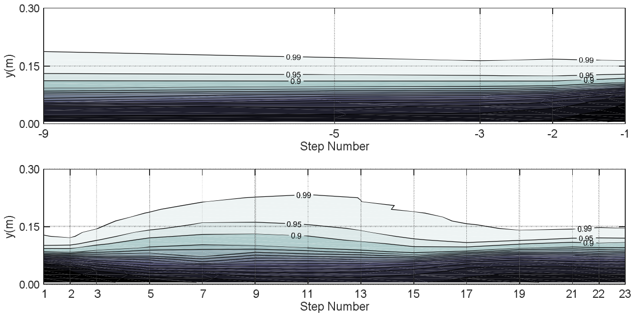
Figure 7. Typical air concentration contour: a) upstream, and b) downstream of the slope change for d_s/h = 3.8 ( y is flow depth perpendicular to the pseudo-bottom).
