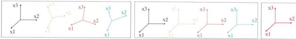
Fig. 5. Left: individual IMUs, each one has its own orientation with respect to the reference IMU (black); Middle: the information is projected into the first reference frame; Right: averaging over the axis gives the synthetic IMU.
