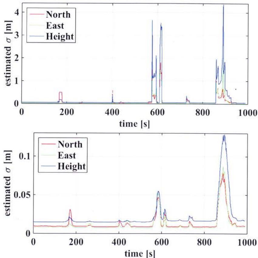
Fig. 4. Standard deviation of the estimated position. Top: GNSS only. Bottom: high-end carrier-phase differential GNSS/INS. The two peaks around time 600 s and 900 s correspond to spots with less favourable satellite reception (Fig. 2 for comparison)
