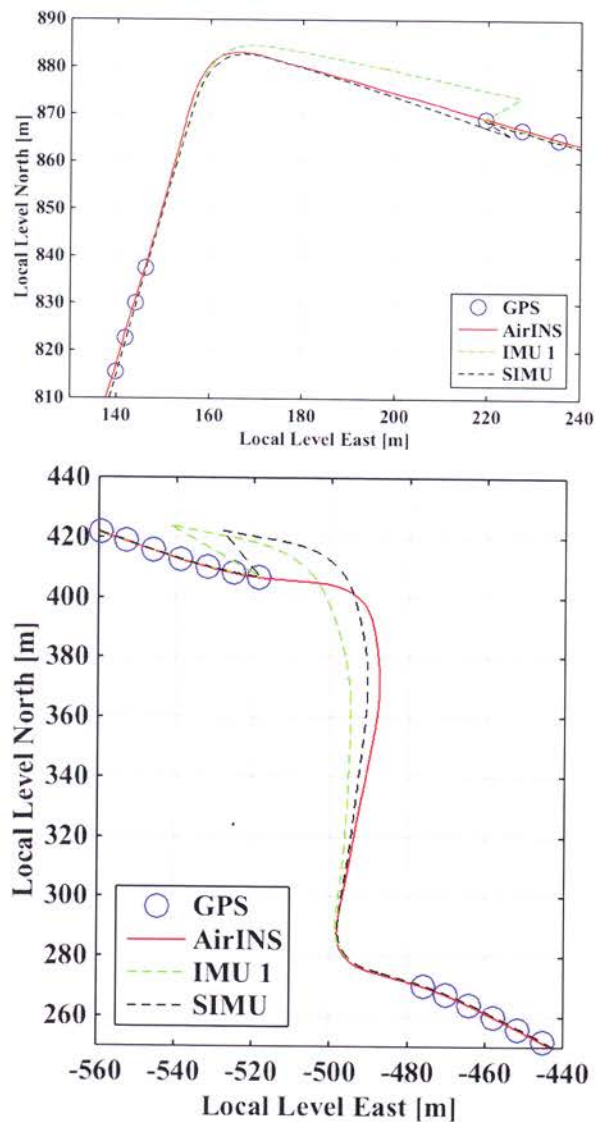
Fig.6. Top: The car turns right without GNSS for 14 s and the IMUs drift away. Bottom: The car enters an S-shaped curve with a 30 s gap in the GNSS data, where the IMUs drift a lot.
