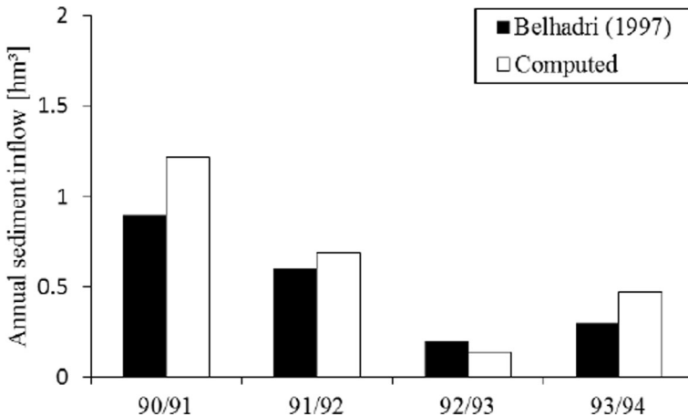
Fig. 3 Comparison between computed annual sediment inflow and values estimated by Belhadri (1997)
