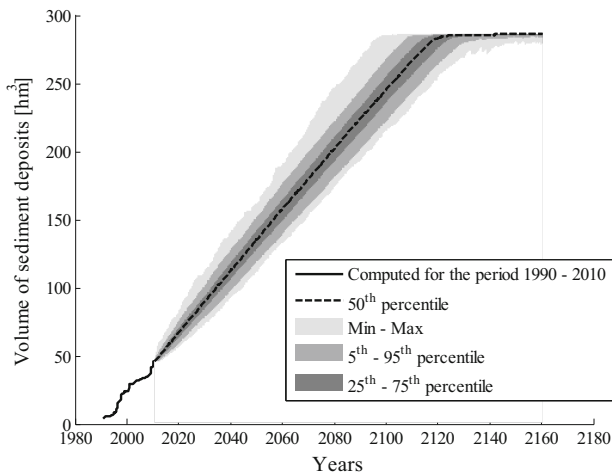
Fig. 7 Long term time evolution of the volume of sediment deposits
