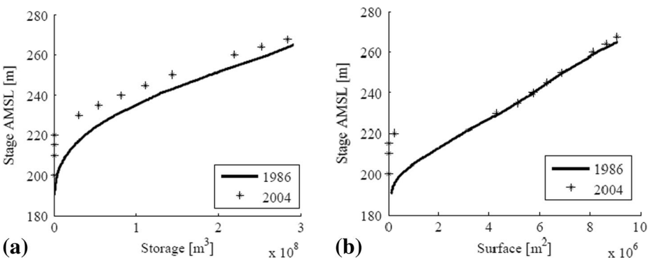
Fig. 2 Stage-storage (a) and stage-surface (b) relationships for the reservoir in 1986 and 2004
