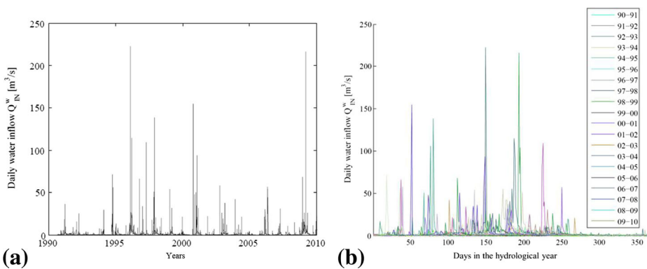
Fig. 4 Computed daily water inflow during the reference period 1990–2010, displayed for the whole period (a) and per hydrological year (b)
