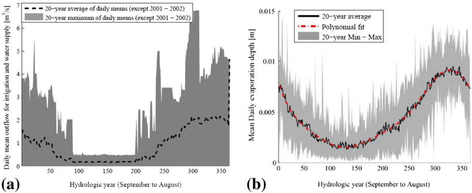
Fig. 1 Daily outflow for irrigation and water supply (a), and daily evaporation depths (b) during the reference period (1990–2010)
