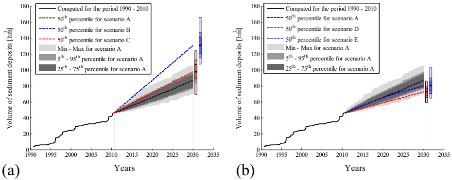
Fig. 8 Time evolution of the volume of sediment deposits for different climate scenarios (a) and different scenarios of erosion control measures in the watershed (b)
