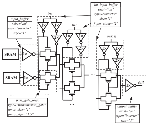
Fig. 6. An example of the transistor-level design of a LUT
