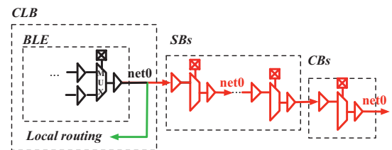
Fig. 9. An example for parasitic nets estimation.
