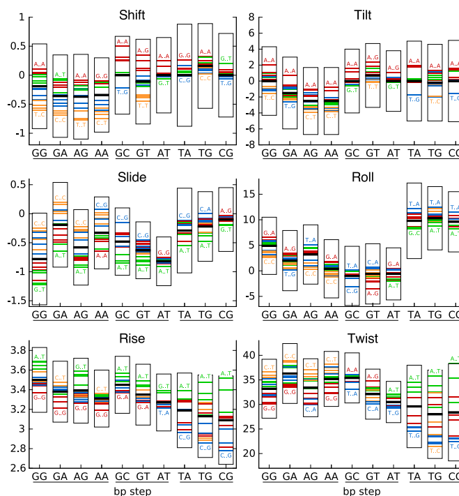
Figure 1. Tetranucleotide sequence effects on inter base pair helical parameter averages. For each parameter, the average value and the standard deviation for the 10 distinct dinucleotide steps (along the abscissa, underlined to show the RR, RY and YR families) are shown by the thick black horizontal lines and surrounding boxes. The impact of the flanking base pairs on each of these values is shown by the colored horizontal lines: R..R (red), R..Y (green), Y..R (blue), and Y..Y (orange). The extreme values of the averages for each dinucleotide step are indicated by the corresponding flanking sequences.
