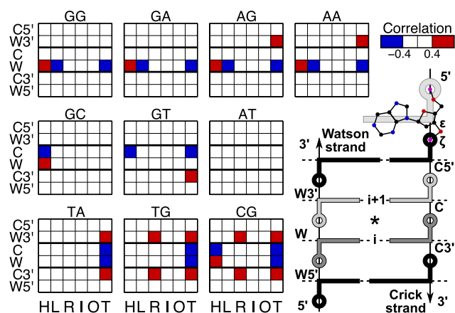
Figure 7. Partial cross correlation matrices between helical parameters and the \zeta (O3'-P) backbone torsion. Cross correlations of the inter-BP parameters, shift (H), slide (L), rise (R), tilt (I), roll (O) and twist (T) and backbone torsion \zeta are shown at three consecutive levels, grouped according to the central dinucleotide step. Positive correlations >0.4 are shown in red and negative correlations <-0.4 are shown in blue. The schematic representation of a double-stranded tetranucleotide fragment on the right defines the naming convention for the \zeta torsions and the six backbone segments: inter-BP parameters refer to the central junction (*) and are grouped according to the dinucleotide sequence at levels i and i+1 on the Watson strand.
