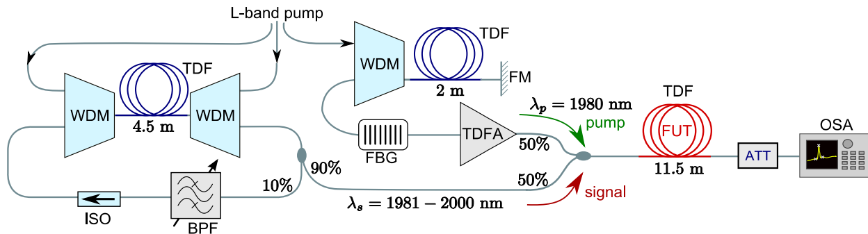
Fig. 1: Experimental setup. WDM: wavelength division multiplexer; ISO: optical isolator; BPF: tunable band-pass filter; FM: fiber mirror; FBG: fiber Bragg grating; TDFA: thulium-doped fiber amplifier; FUT: fiber under test; OSA: optical spectrum analyzer; ATT: fixed attenuator
