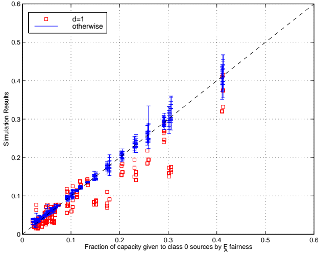
Fig. 4. HOMRTT with the stolen lag, \tau_i = 0.2 s, r_i = 5 , \eta_i = 0.5 for all flows.
