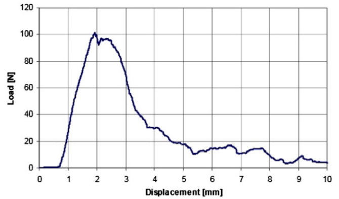
Fig. 5. Typical load/displacement plot.
