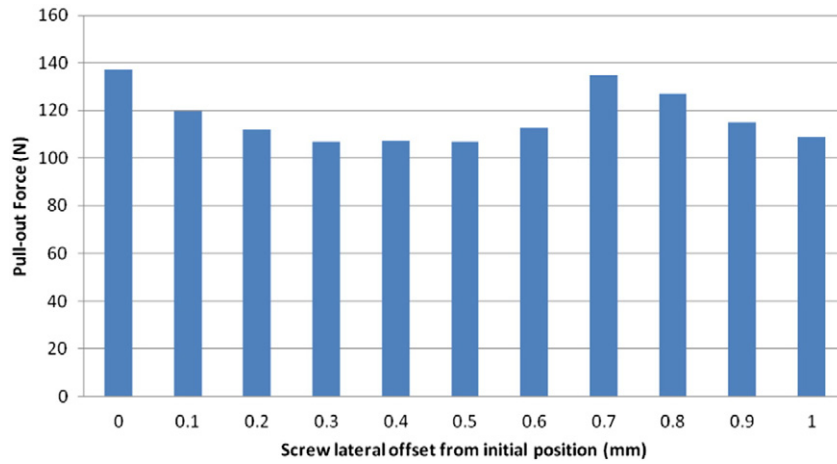
Fig. 8. Variation in pullout force with lateral position from FE model.
