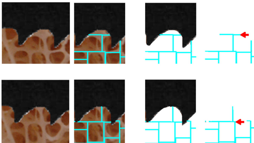
Fig. 9. Interdigitation model.
