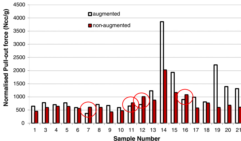
Fig. 4. Pullout force normalised for bone density.
