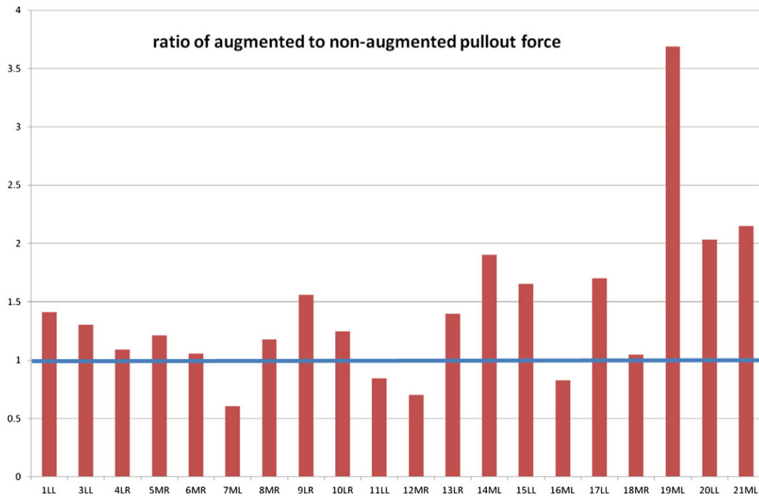
Fig. 6. Ratio of augmented to non-augmented normalised pullout force.
