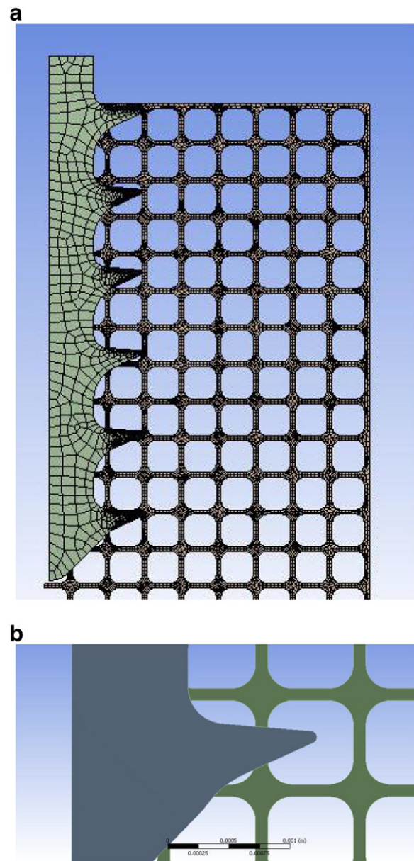
Fig. 3. Simplified finite element model showing mesh (a) and tooth engagement (b).
