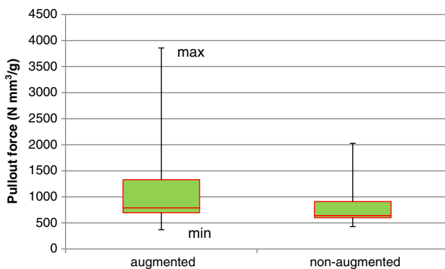
Fig. 7. Box plot of minimum, Q1, mean, Q3, and maximum.
