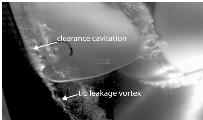
Figure 1. Tip leakage vortex and clearance cavitation in a bulb turbine reduced scale model.
