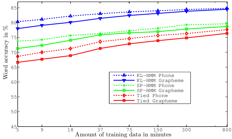
(b) on the Greek ASR task.
