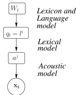
Figure 2: The graphical model representation of a deterministic lexical model based ASR system.
