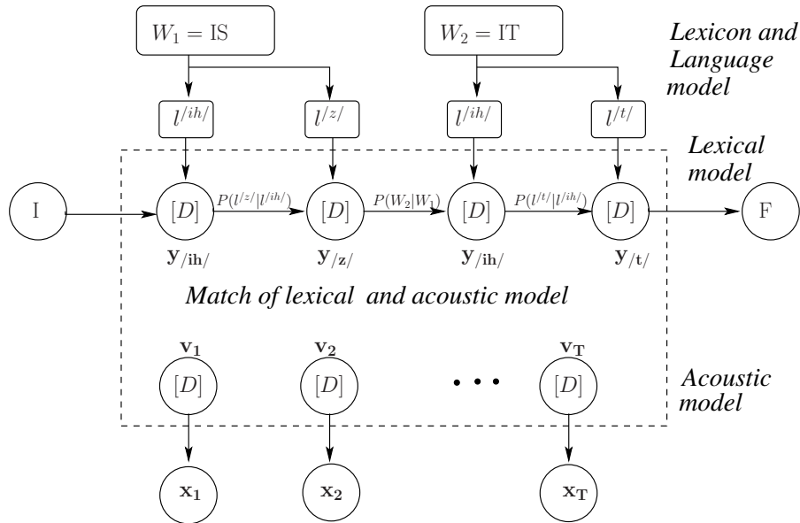
Figure 1: The graphical model representation of a system incorporating probabilistic lexical modeling.
