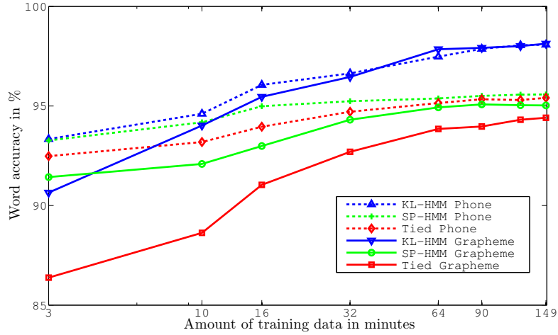
(a) on the HIWIRE non-native accented speech recognition task.
