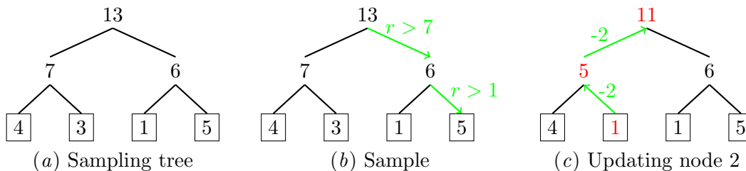
Figure 3: Sampling according to a changing discrete distribution — Given a binary tree build on top of a discrete distribution [4, 3, 1, 5]/13 (3(a)), we can draw a sample according to this distribution by recursively sampling according to the partial distribution of the children at a given node (2.3). Only the nodes between the leaf to update and the root need to be updated (2.3). Both operations have \mathcal{O}(\log N) complexity.
