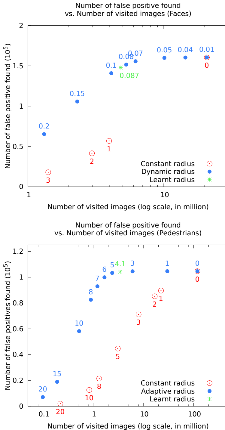
Figure 4: Number of false positives found vs. the number of visited samples for the different strategies (average over 10 runs) — In the experiments, we visit the scenes until all are exhausted. The red circles correspond to a strategy which discards a disc of constant radius around a visited sample x , the blue dots to the strategy which uses an adaptive radius -af_1(x) . The learnt radius (green star) is in the area where almost all the available false positives are found while visiting a minimum of positions.
