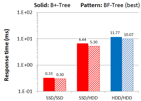
Figure 7: BF-Tree and B^+ -Tree with warm caches
