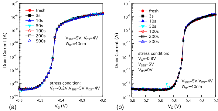
Fig.11. Reliability assessment during fast transition ( SS < 10 mV/dec): (a) hot carrier injection and (b) bias temperature instability with different stress period. No significant degradation is observed, proving the good reliability of the device.
