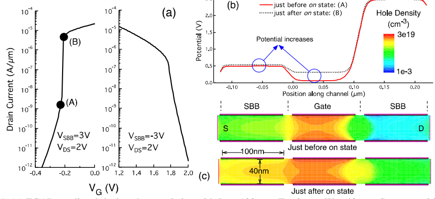
Fig.4. (a) TCAD-predicted device characteristics with L_{gate}=100 nm, T_{ox}=2 nm, W_{fin}=40 nm. Steep transition is observed in both n -type ( \sim 5 mV/dec) and p -type ( \sim 35 mV/dec). The device polarity changes by adapting the polarity of V_{SBB} . (b) Surface potential distribution just before and after on state ( n -type). Potential increases under both Gate and SBB. (c) Hole density showing the accumulation of holes under Gate and SBB.
