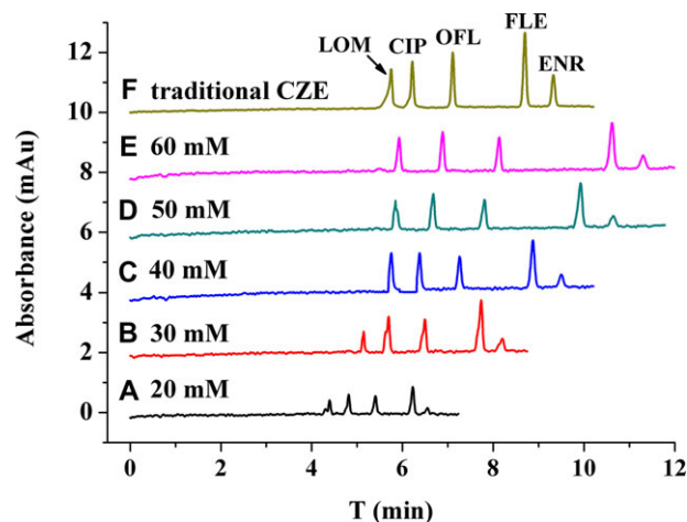
Figure 1. (A)–(E) Effect of BGE concentration ranging from 20 to 60 mM on the FESI stacking and CZE separation. (F) Conventional CZE without any sample stacking. FESI-CZE conditions: a standard capillary with total/effective length of 48.5/40 cm and id/od of 50/365 \mu m for separation, water plug injected by a low pressure of 40 mbar for 50 s, sample mixture of five FQs at a concentration of 25 ng/mL for each compound was injected by a high voltage of -8 kV for 4 min, separated at 30 kV and detected at 280 nm. Conventional CZE conditions: sample of FQs at a concentration of 5 \mu g/mL and injected by a pressure of 35 mbar for 40 s, others same with those of FESI-CE.
