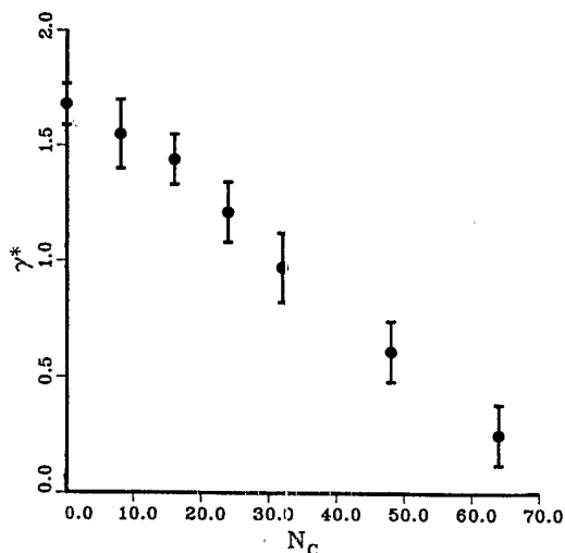
FIG. 4. The reduced surface tension \gamma^* = \gamma \sigma^2 \epsilon^{-1} of the liquid-liquid interface as a function of total number of amphiphiles ( N_C ).
