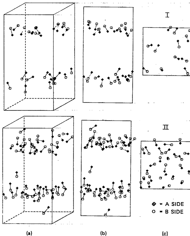
FIG. 3. Snapshot of the positions of the amphiphiles. (Note that the positions of particles A and B of the bulk liquids are not drawn.) In (a) a perspective view is given, in (b) a projection on the front plane, and in (c) a projection of the lower layer on the bottom plane. The total number of amphiphiles is 24 (I) and 48 (II).
