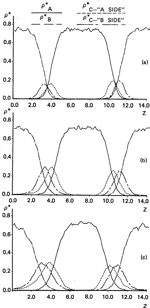
FIG. 2. Density profiles of compounds A , B , and C as a function of the height z . In order to demonstrate the ordering of the amphiphiles ( C ), the density profiles of the "A side" and "B side" of the amphiphiles are drawn separately. The total number of amphiphiles is (a) N_C = 24 , (b) N_C = 48 , (c) N_C = 64 .
