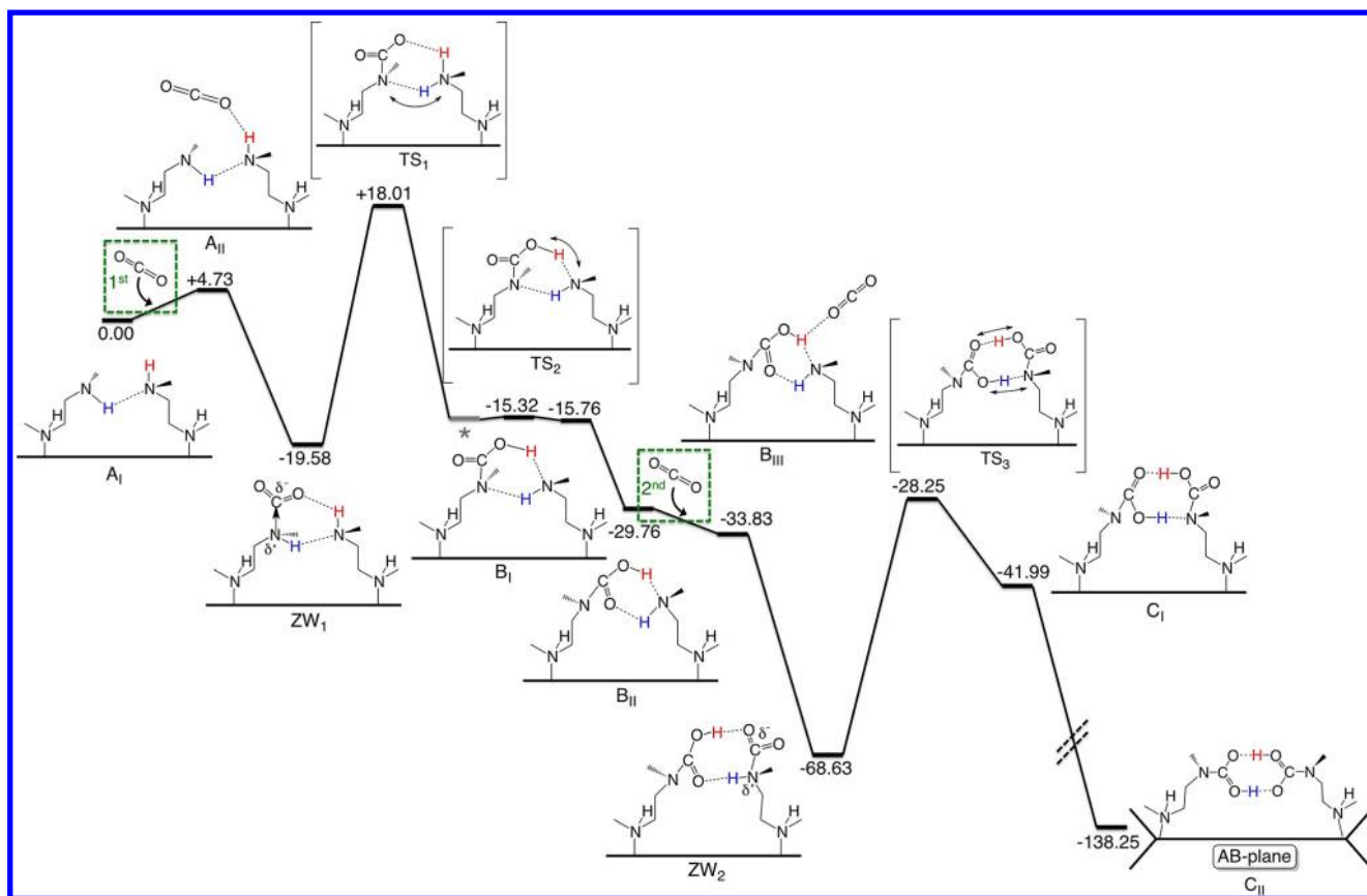
Figure 2. The proposed mechanism: (left) first \text{CO}_2 uptake ( \text{CO}_2 :amine = 1:2); (right) second \text{CO}_2 uptake ( \text{CO}_2 :amine = 2:2). The energy profile, \Delta E , reported in \text{kJ}/(\text{mol of model fragment}) , was calculated as \Delta E = E_{\text{species}} - E_{A_I} - nE_{\text{CO}_2} where n = 1 (first uptake) or 2 (second uptake). The dashed diagonal lines indicate that the \Delta E of species C_{II} is not drawn to scale. Coordinates and energies of all optimized species are given in sections 8–9 in the SI.
