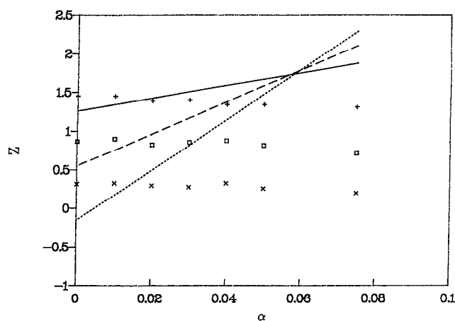
FIG. 3. Compressibility factor Z for polarizable Lennard-Jones/Stockmayer mixtures. Symbols as in Fig. 2
