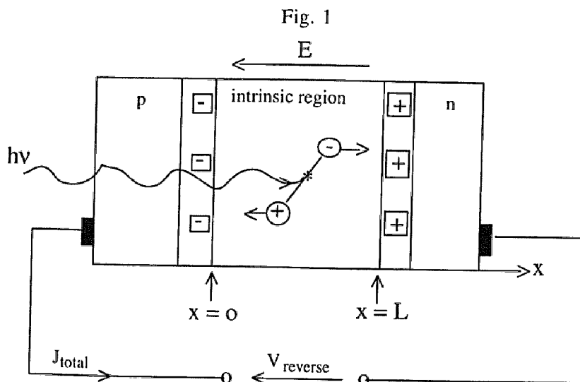
p - i - n solar cell under reverse voltage. x is the position in the i layer. At x = 0 is the p - i interface and x = L is the i - n interface. V_{reverse} is the external applied voltage. E is the electric field in the i layer due to V_{reverse} and due to the depletion region at the p - i and at the i - n interfaces.
